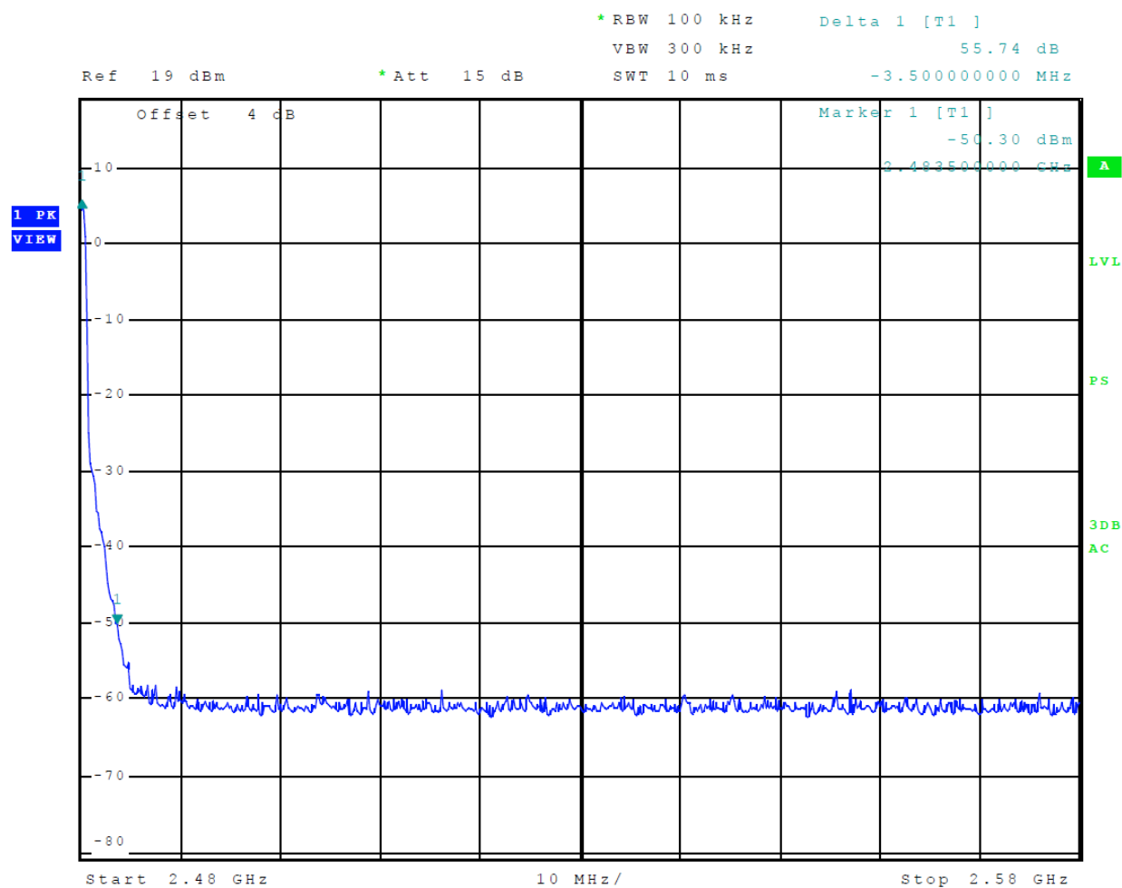
Figure 16 Plot of Transmitter Emissions High Band Edge Mode 3 (PI/4 DPQSK)
