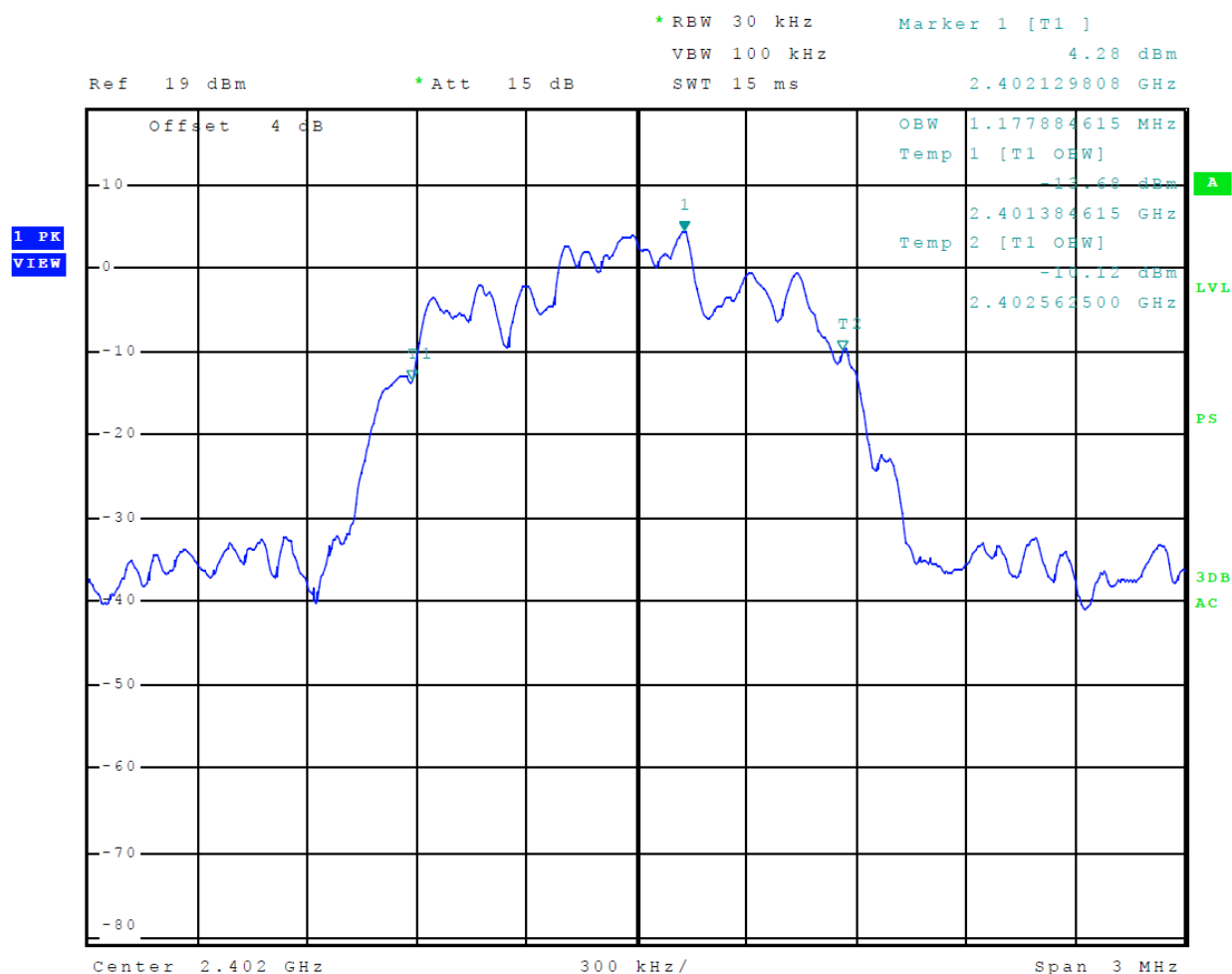
Figure 10 Plot of Transmitter Emissions 99% Occupied Bandwidth Mode 2 (GFSK)
