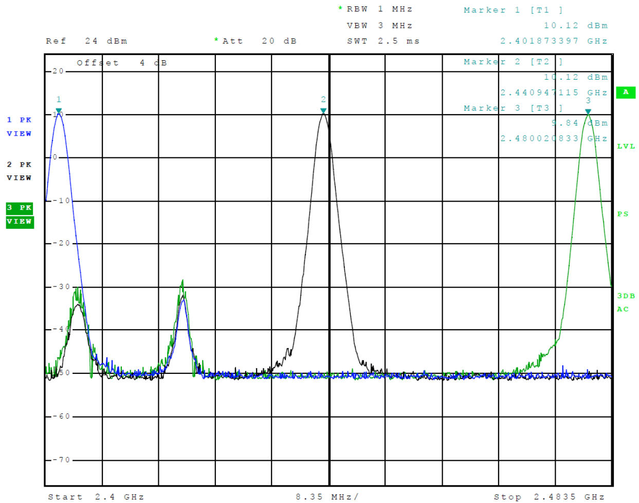
Figure 9 Plot of Transmitter Emissions Operation in 2402-2480 MHz Mode 2 (GFSK)
