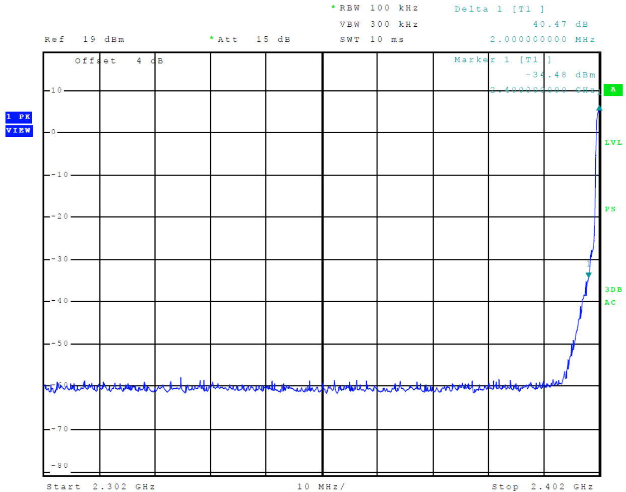
Figure 15 Plot of Transmitter Emissions Low Band Edge Mode 3 (PI/4 DPQSK)
