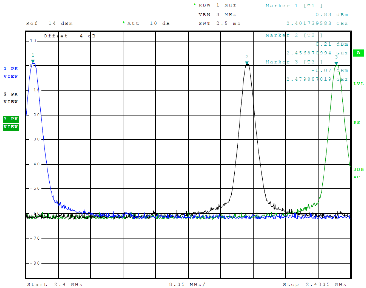
Figure 5 Plot of Transmitter Emissions Operation in 2402-2480 MHz Mode 1 (GFSK)
