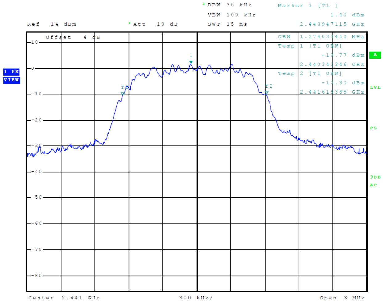
Figure 14 Plot of Transmitter Emissions 99% Occupied Bandwidth Mode 3 (PI/4 DPQSK)
