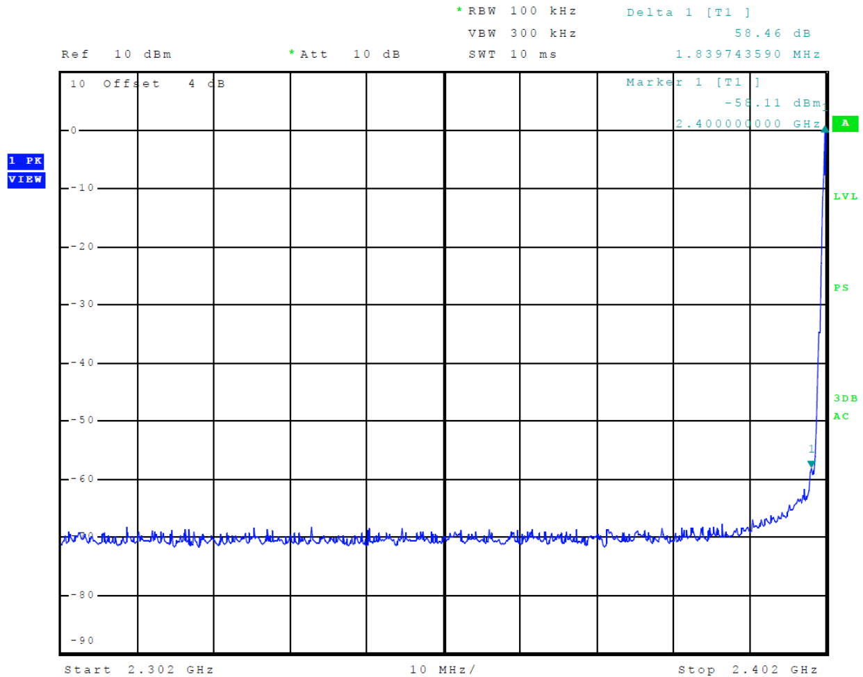
Figure 7 Plot of Transmitter Emissions Low Band Edge Mode 1 (GFSK)
