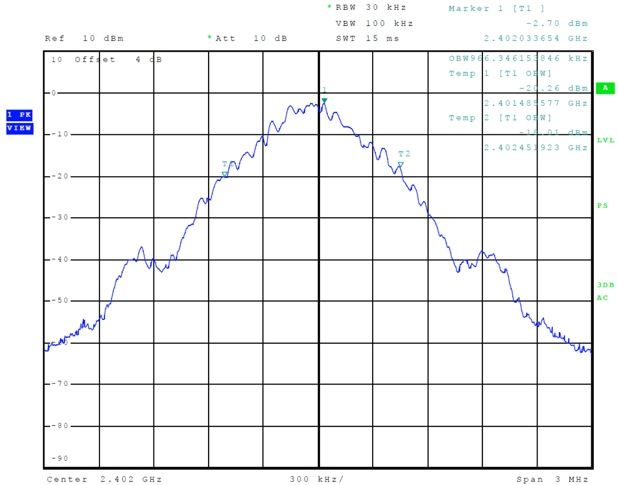
Figure 6 Plot of Transmitter Emissions 99% Occupied Bandwidth Mode 1 (GFSK)
