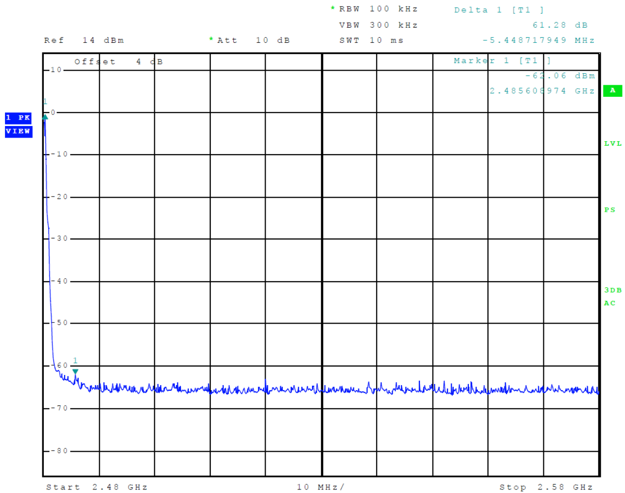
Figure 20 Plot of Transmitter Emissions High Band Edge Mode 4 (GMSK)
