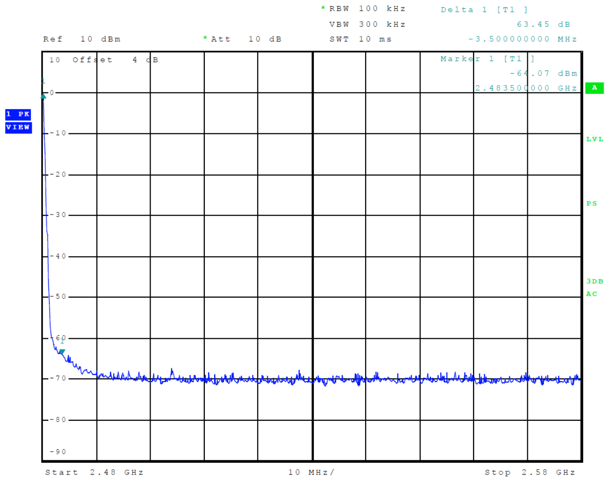
Figure 8 Plot of Transmitter Emissions High Band Edge Mode 1 (GFSK)
