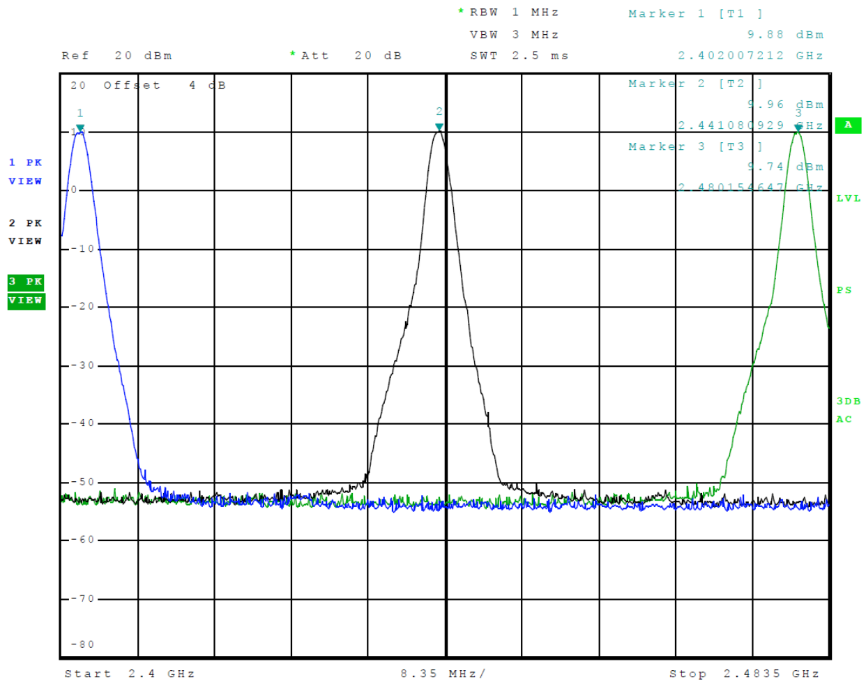
Figure 13 Plot of Transmitter Emissions Operation in 2402-2480 MHz Mode 3 (PI/4 DPQSK)
