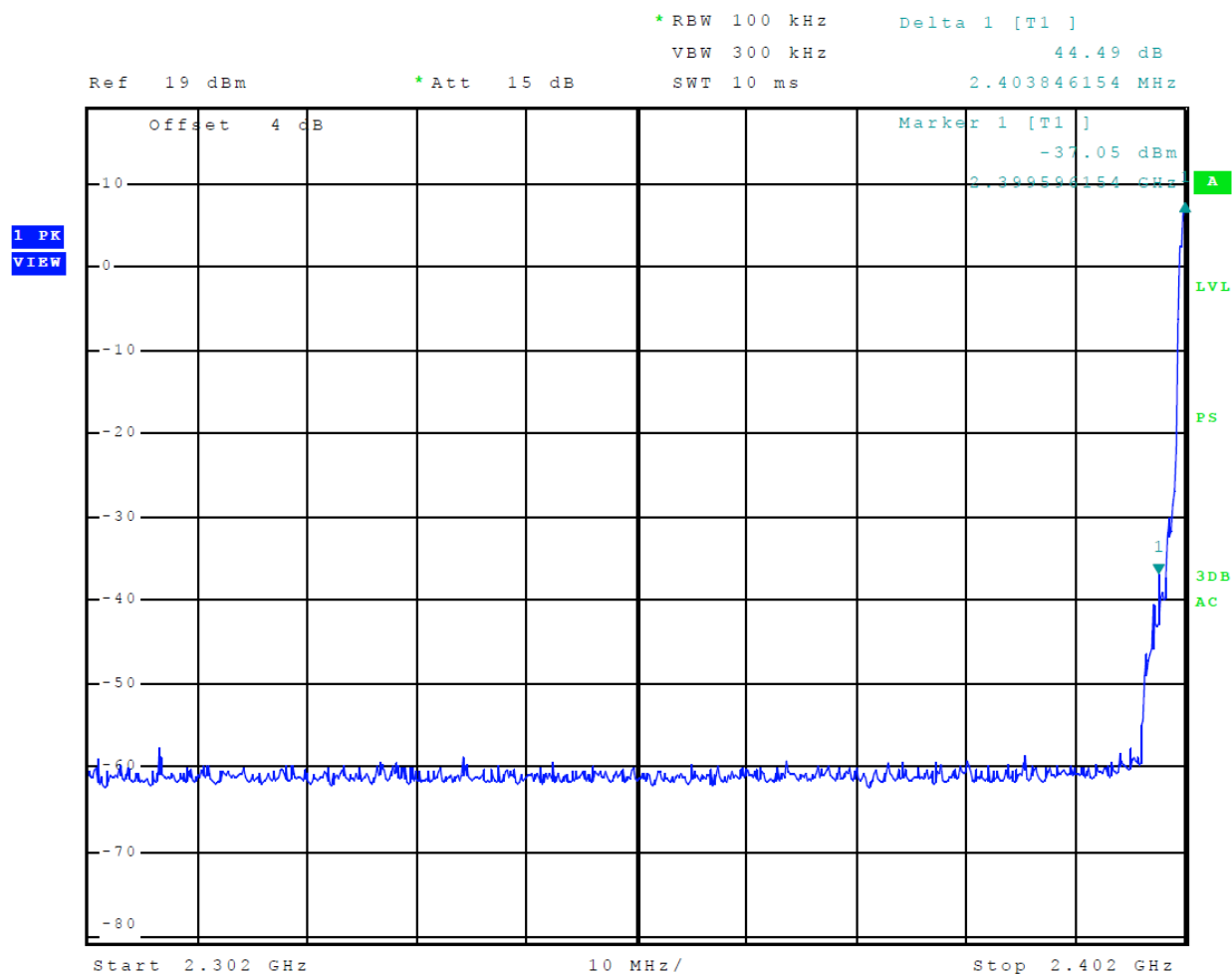
Figure 11 Plot of Transmitter Emissions Low Band Edge Mode 2 (GFSK)
