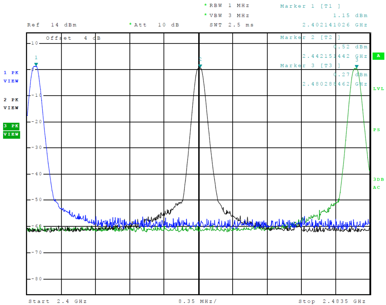
Figure 17 Plot of Transmitter Emissions Operation in 2402-2480 MHz Mode 4 (GMSK)
