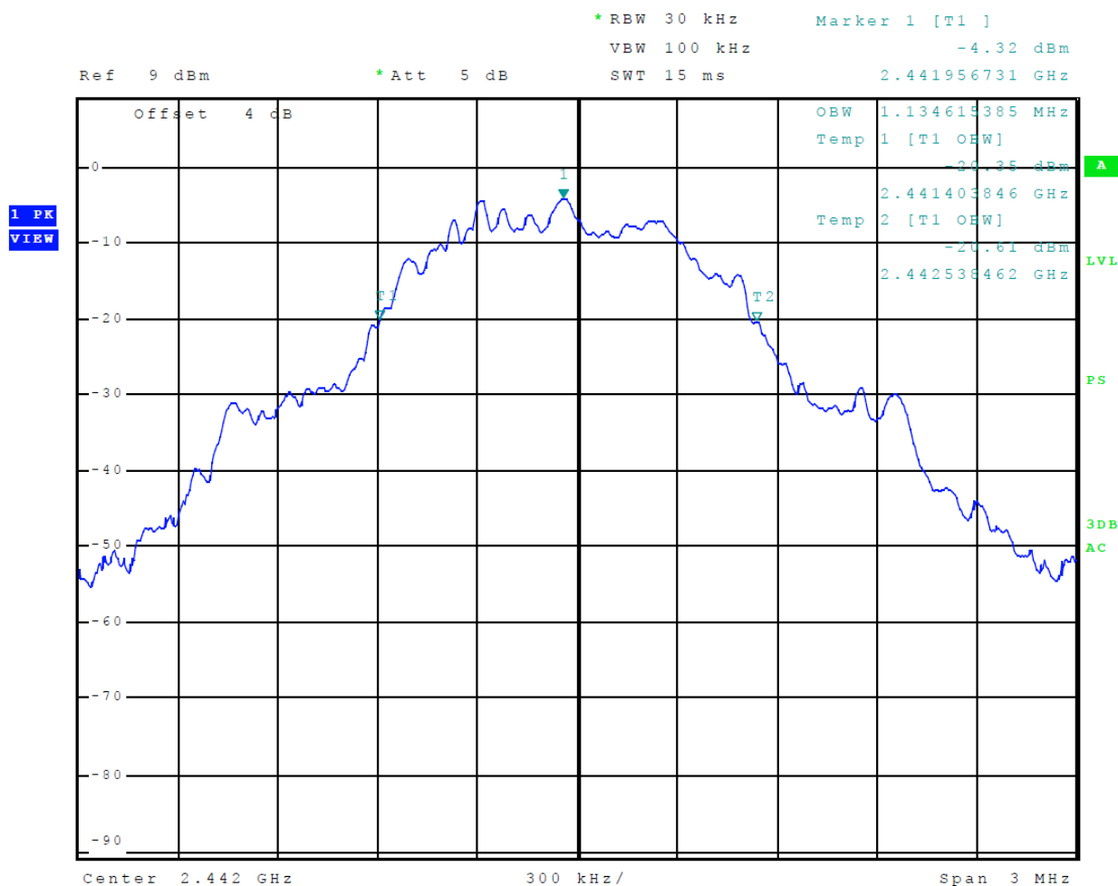
Figure 18 Plot of Transmitter Emissions 99% Occupied Bandwidth Mode 4 (GMSK)
