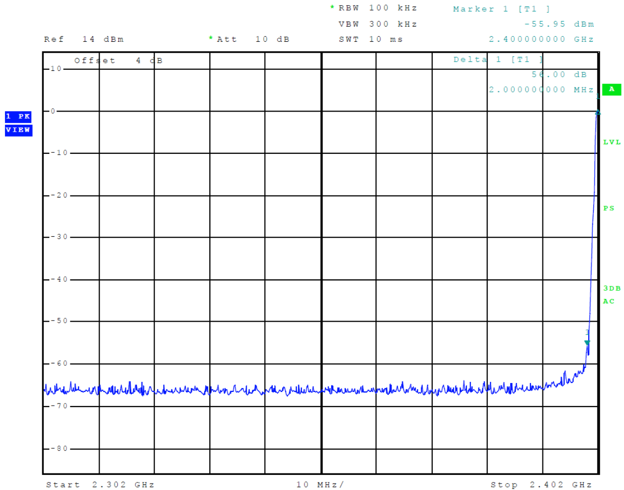
Figure 19 Plot of Transmitter Emissions Low Band Edge Mode 4 (GMSK)
