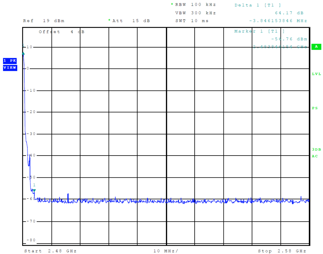
Figure 12 Plot of Transmitter Emissions High Band Edge Mode 2 (GFSK)
