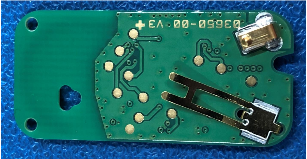
Figure 2 - PCB, Bottom
