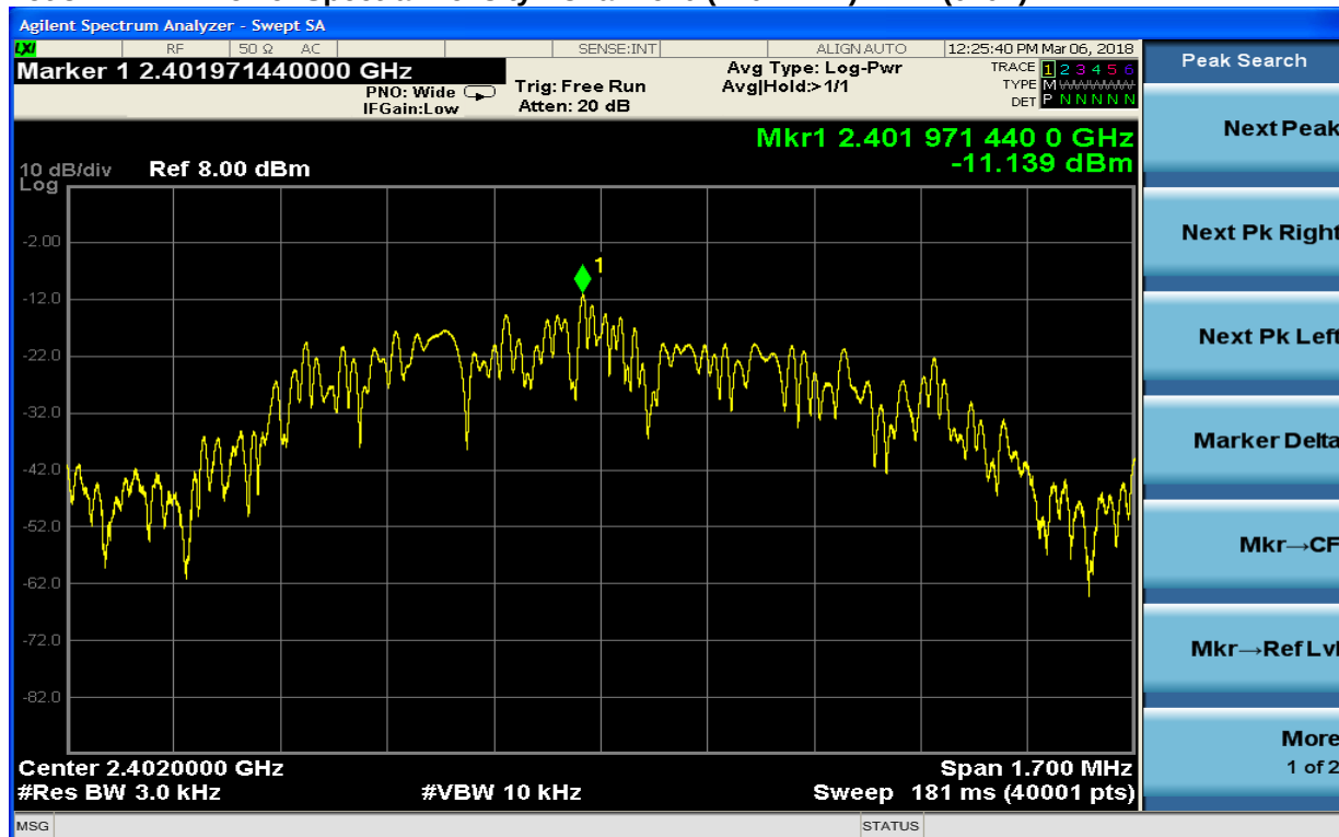
Plot 8-7: Power Spectral Density: Channel 0 (2402 MHz): BLE (0x0F)
