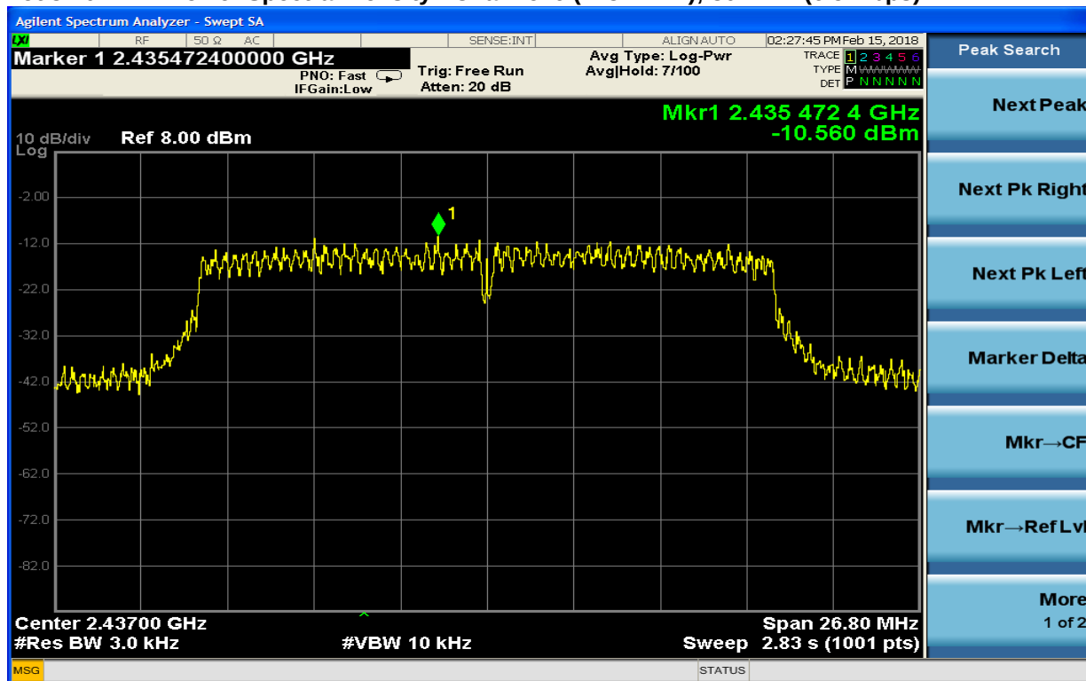
Plot 8-20: Power Spectral Density: Channel 6 (2437 MHz); 802.11n (6.5 Mbps)
