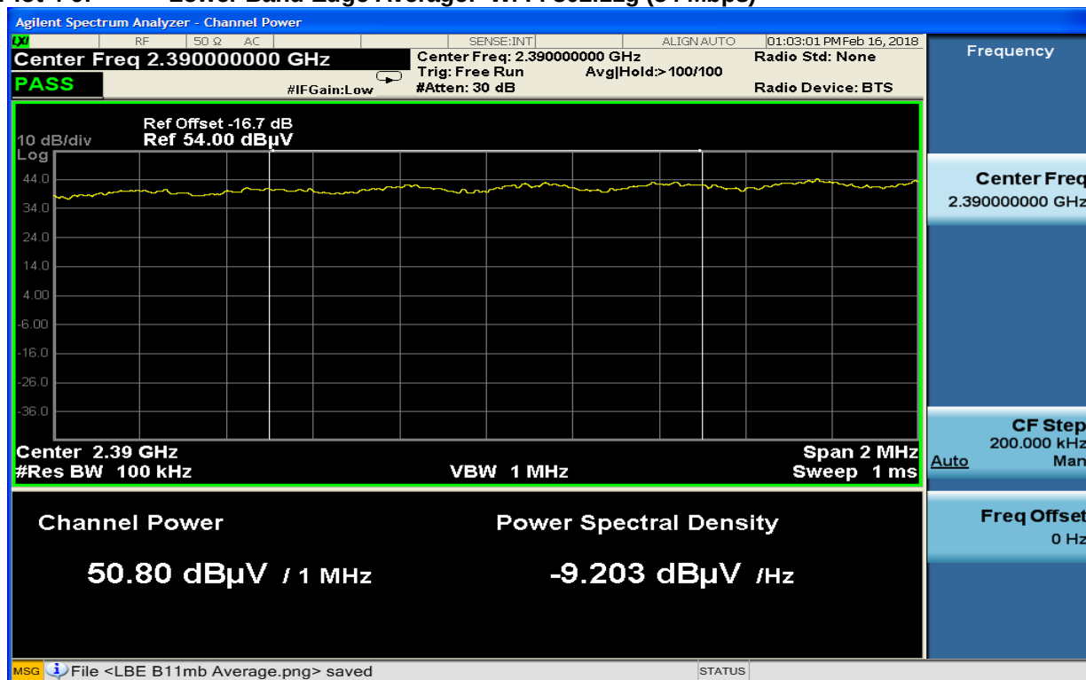
Plot 4-9: Lower Band Edge Average: Wi Fi 802.11g (54 Mbps)
