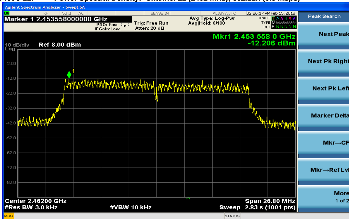
Plot 8-21: Power Spectral Density: Channel 11 (2462 MHz); 802.11n (6.5 Mbps)
