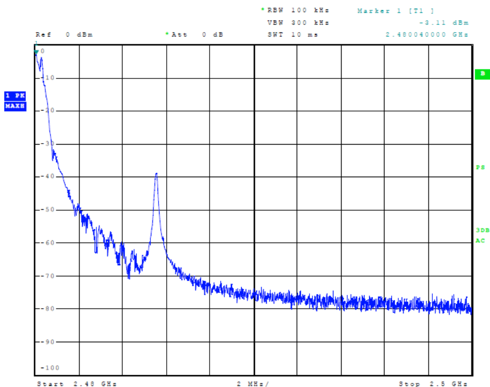
Figure 10 Plot of Transmitter Emissions (High Band Edge)
