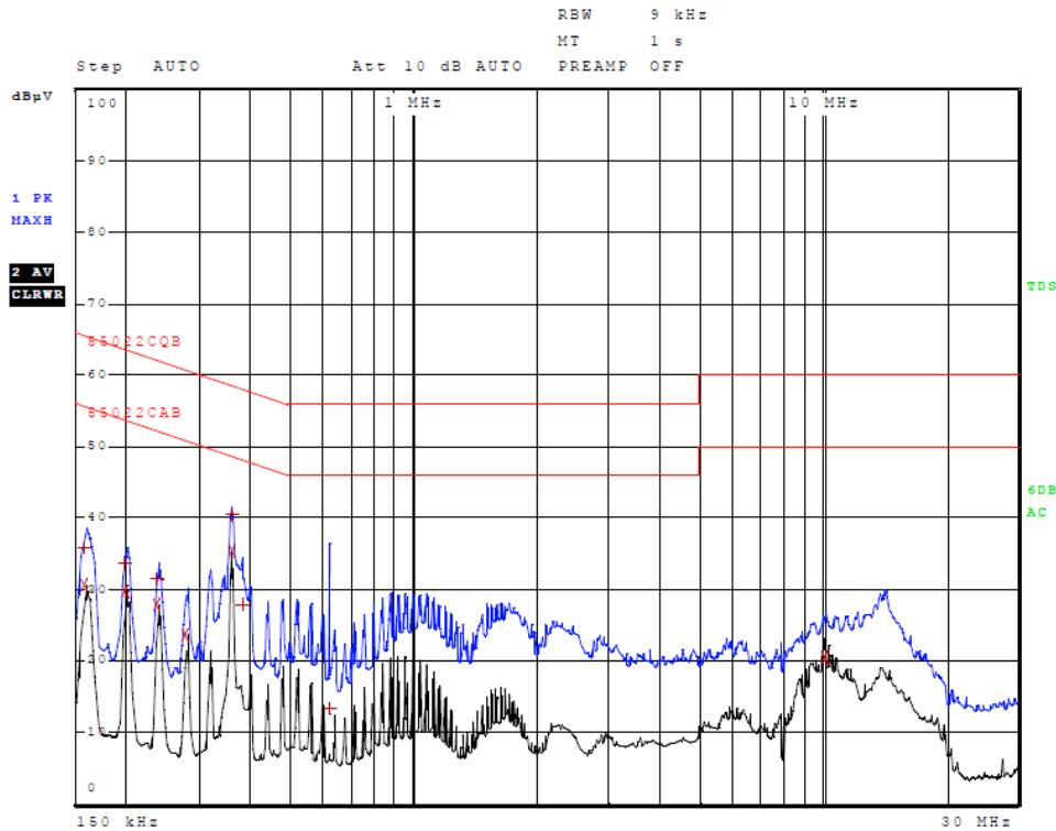
Figure 1 AC Line Conducted emissions of EUT line 1 (EUT AC Adapter 326-00072-00)
