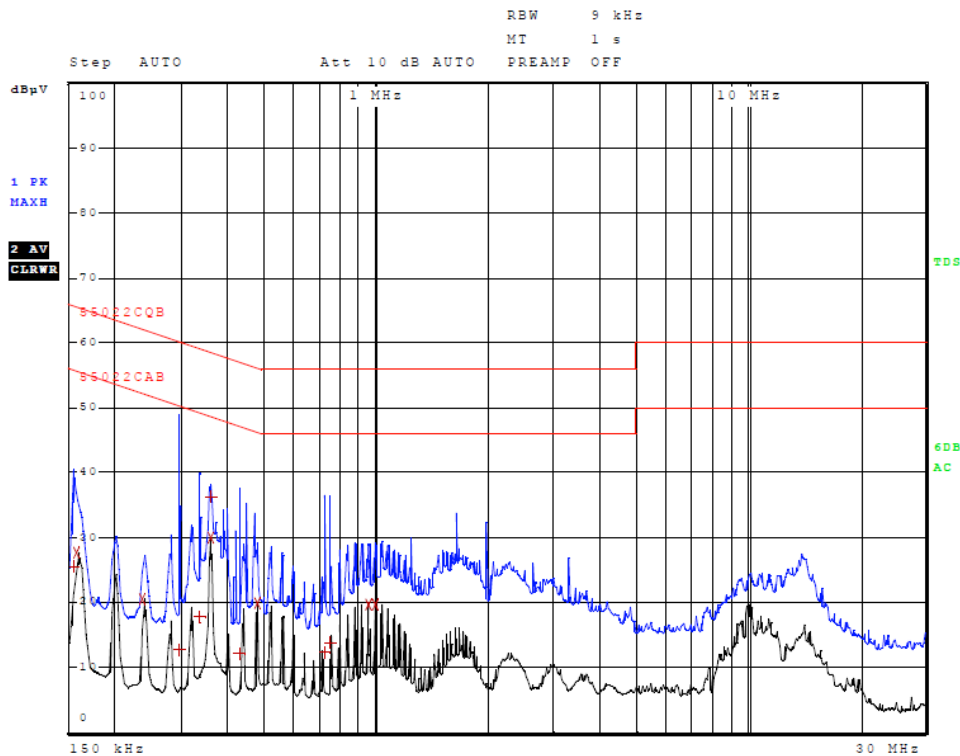
Figure 2 AC Line Conducted emissions of EUT line 2 (EUT AC Adapter 326-00072-00)
