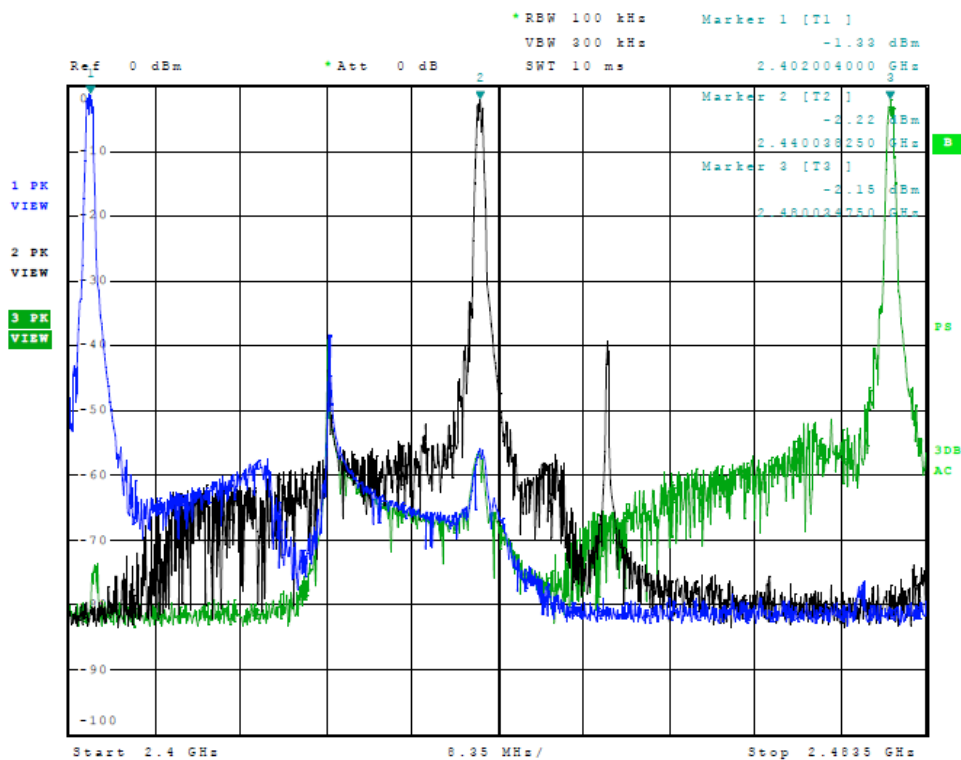
Figure 7 Plot of Transmitter Emissions (In 2402-2480 MHz)
