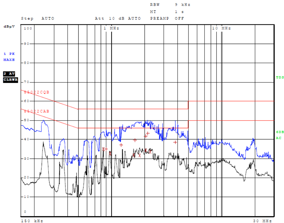
Figure 5 AC Line Conducted emissions of EUT line 1 (EUT-USB-CPU AC Adapter)
