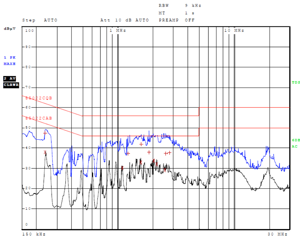
Figure 6 AC Line Conducted emissions of EUT line 2 (EUT-USB-CPU AC Adapter)
