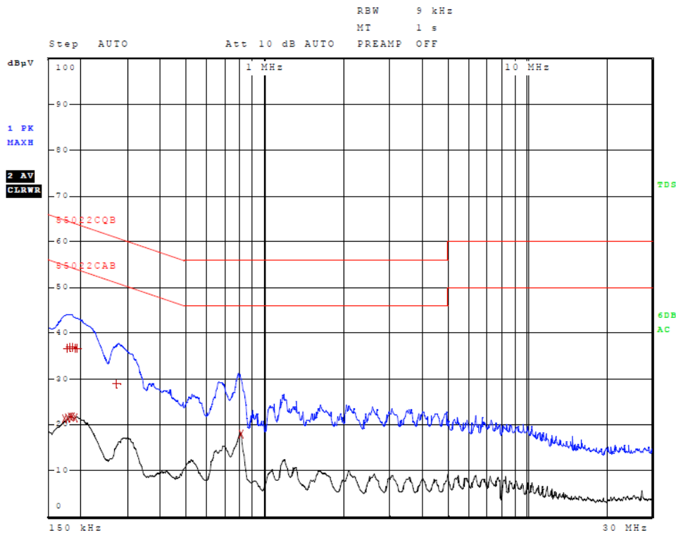
Figure 4 AC Line Conducted emissions of EUT line 2 (EUT AC Adapter 326-00087-00)
