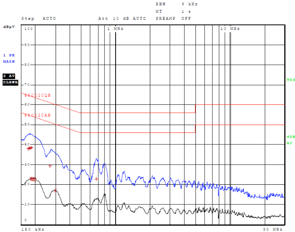
Figure 3 AC Line Conducted emissions of EUT line 1 (EUT AC Adapter 326-00087-00)
