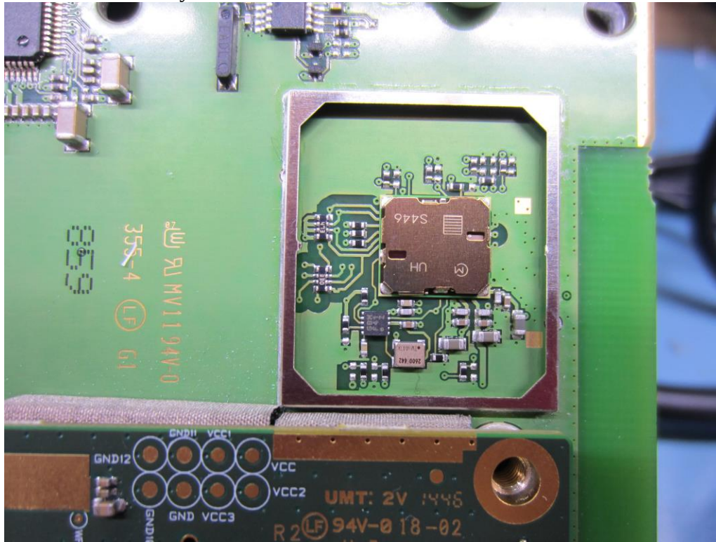
Transmitter circuitry
