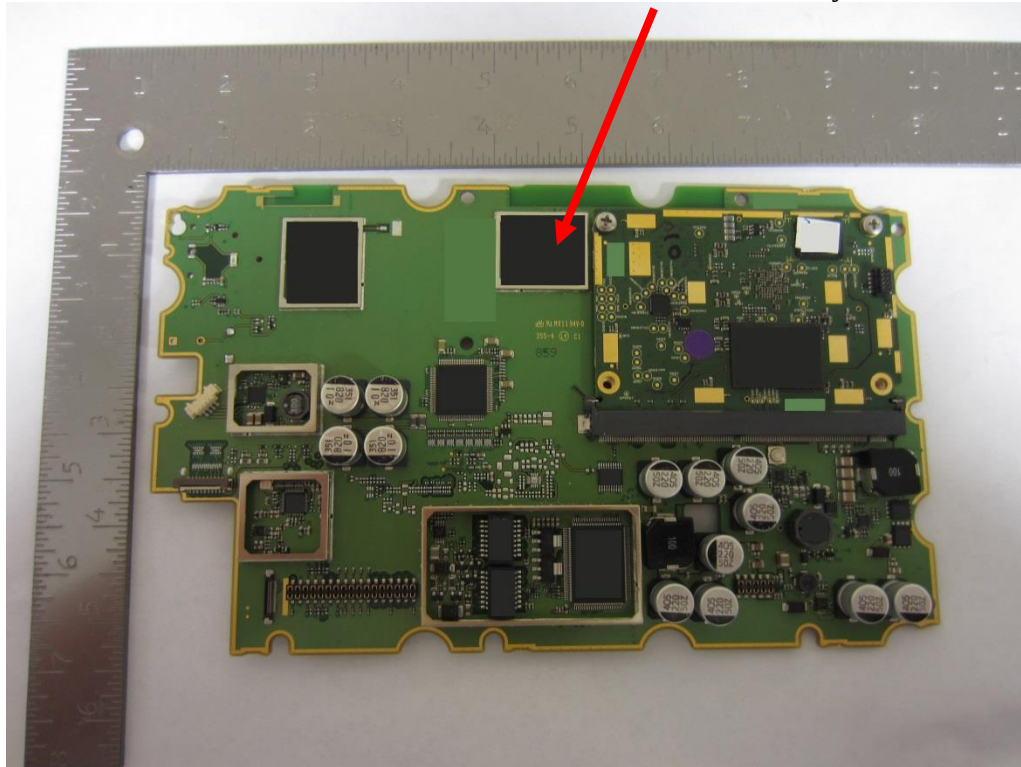
Internal Photographs Main PCB back side
