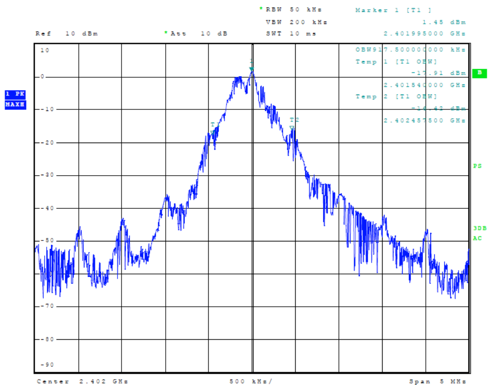
Figure 6 Plot of Transmitter Emissions (99% Occupied Bandwidth, Mode 1)
