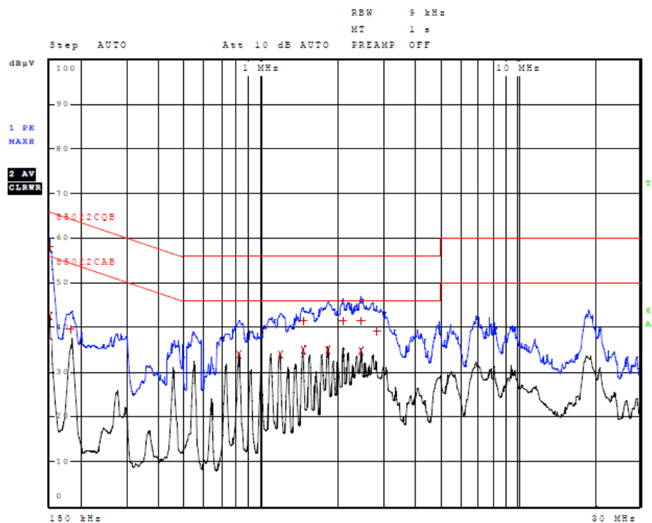
Figure 4 AC Line Conducted emissions of EUT line 2 (EUT-USB-CPU)
