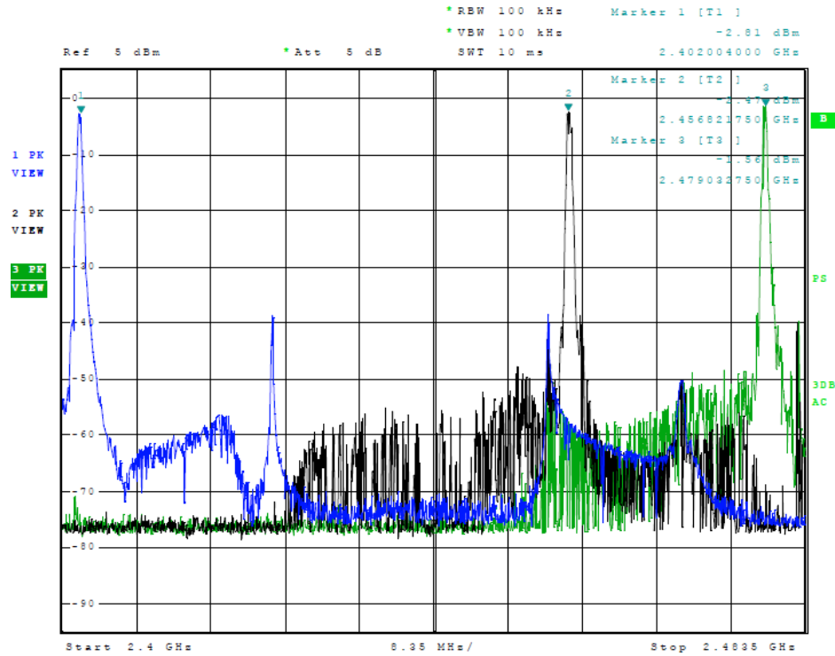
Figure 9 Plot of Transmitter Emissions (In 2402-2479 MHz Band, Mode 2)
