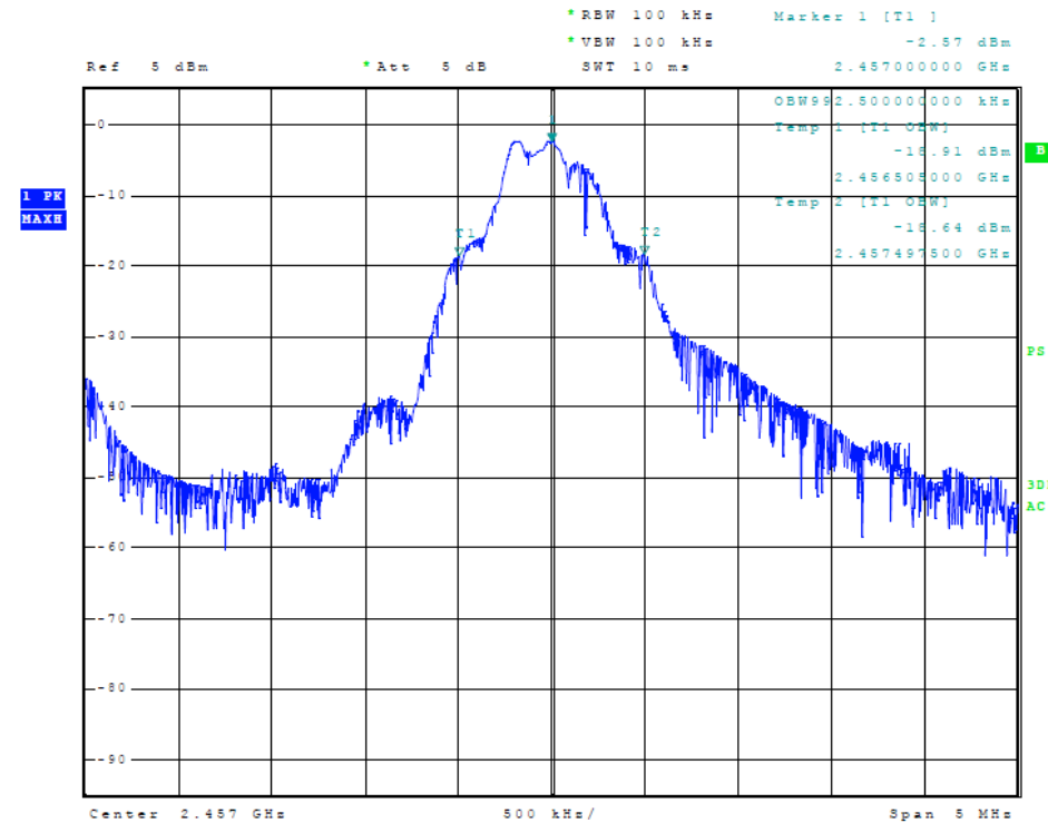
Figure 10 Plot of Transmitter Emissions (99% Occupied Bandwidth, Mode 2)
