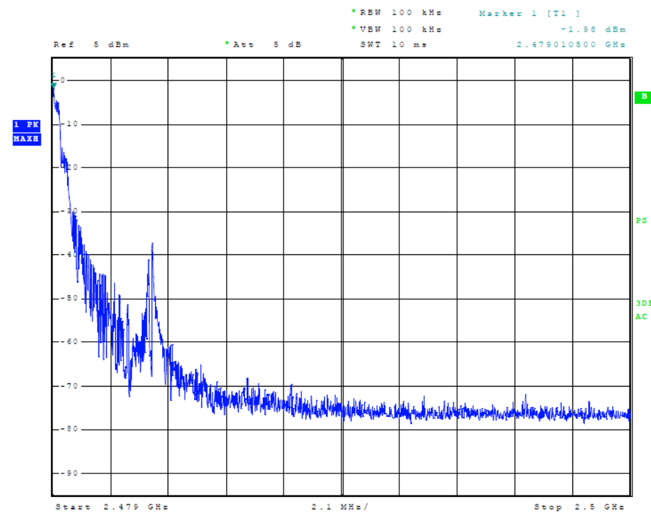
Figure 12 Plot of Transmitter Emissions (High Band Edge, Mode 2)
