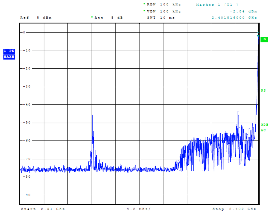
Figure 11 Plot of Transmitter Emissions (Low Band Edge, Mode 2)
