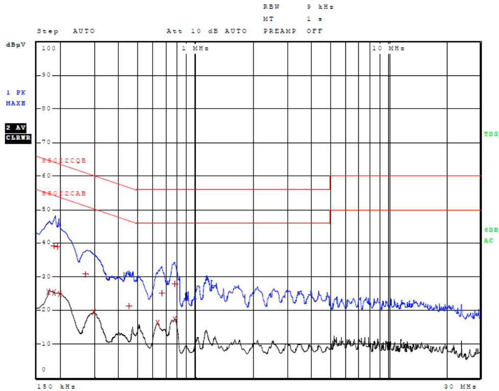
Figure 1 AC Line Conducted emissions of EUT line 1 (EUT AC Adapter #1)
