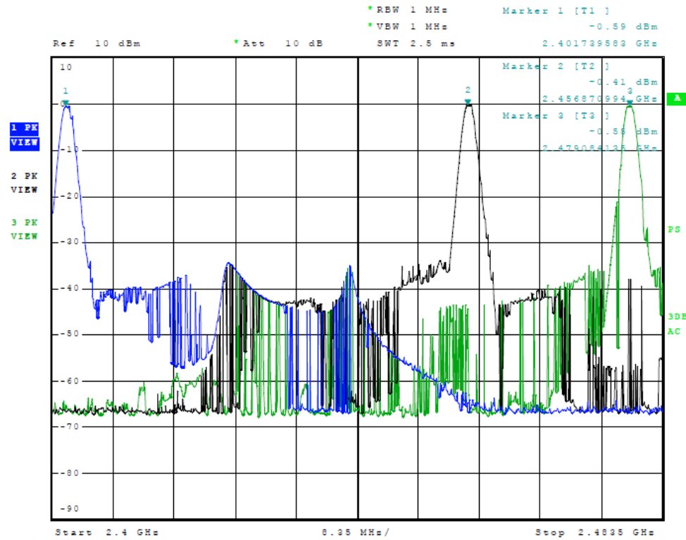
Figure 7 Plot of Transmitter Emissions (In 2402-2480 MHz Band) (Mode 1)
