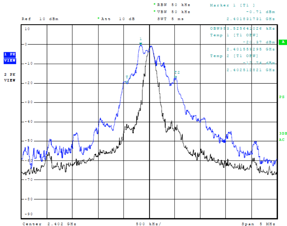
Figure 8 Plot of Transmitter Emissions (99% Occupied Bandwidth) (Mode 1)
