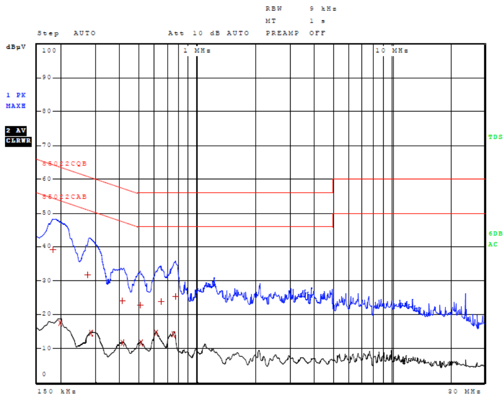
Figure 2 AC Line Conducted emissions of EUT line 2 (EUT AC Adapter #1)
