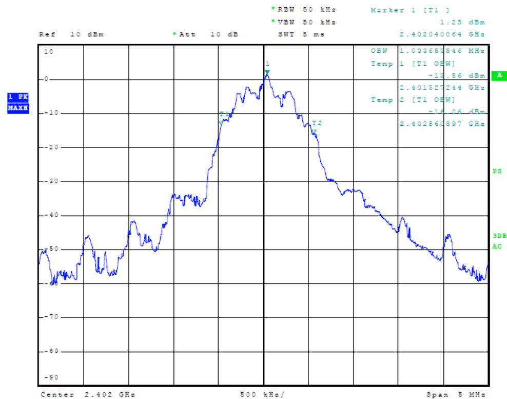
Figure 12 Plot of Transmitter Emissions (99% Occupied Bandwidth) (Mode 2)
