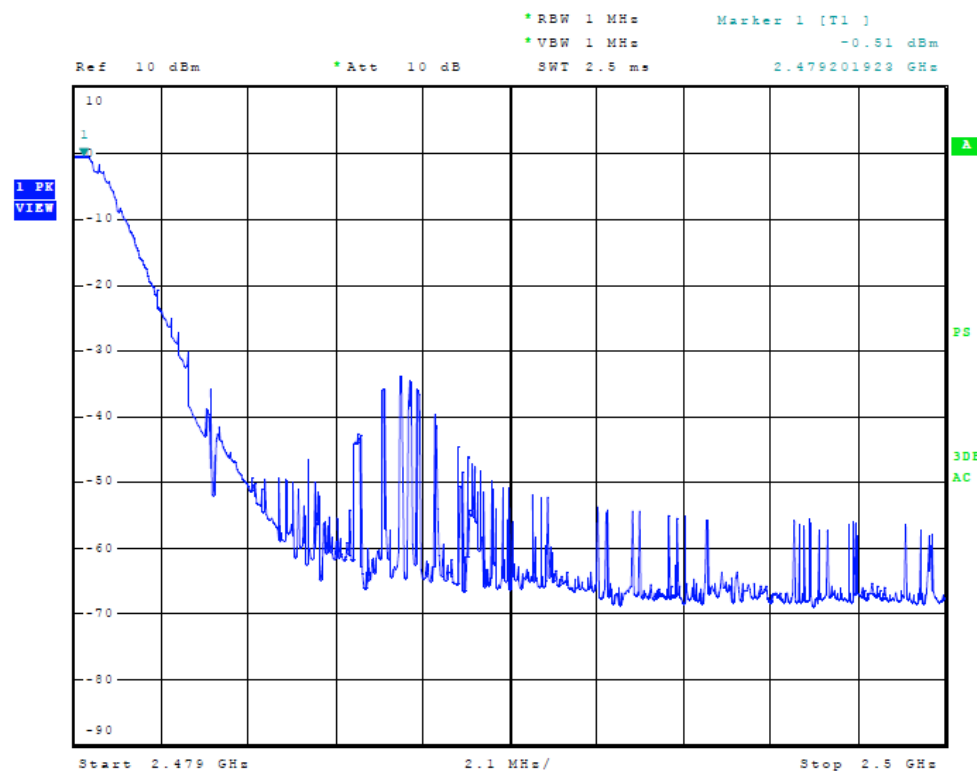
Figure 10 Plot of Low Band Edge (High Band Edge) (Mode 1)
