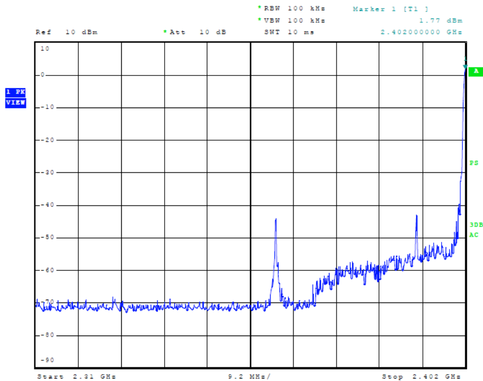
Figure 13 Plot of Transmitter Emissions (Low Band Edge) (Mode 2)
