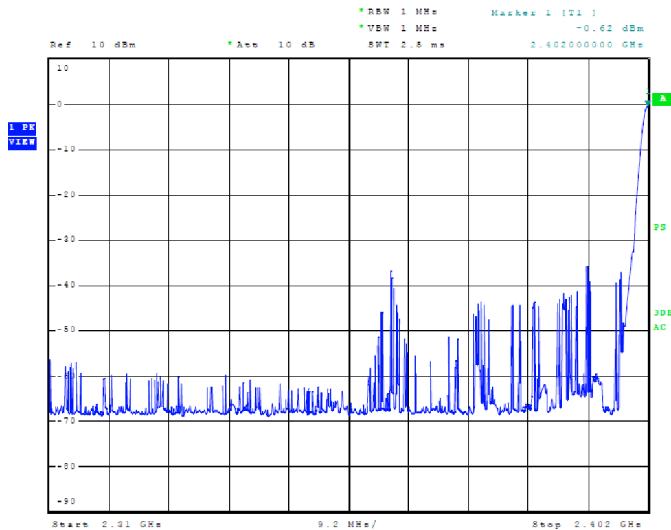
Figure 9 Plot of Transmitter Emissions (Low Band Edge) (Mode 1)
