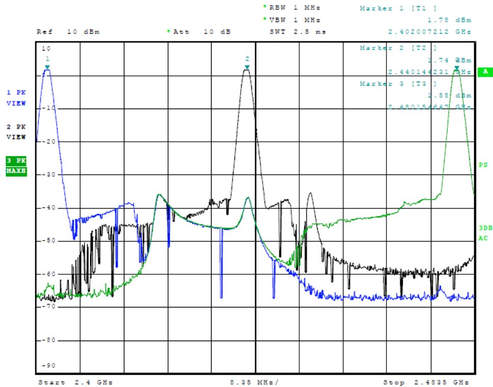
Figure 1 Plot of Transmitter Emissions (In 2402-2480 MHz Band) (Mode 2)
