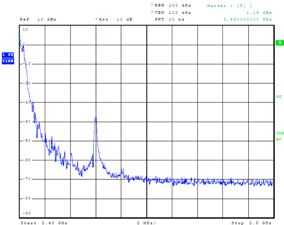
Figure 14 Plot of Low Band Edge (High Band Edge) (Mode 2)
