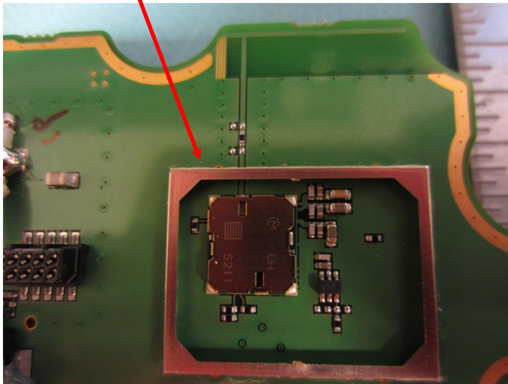
Transmitter Section
