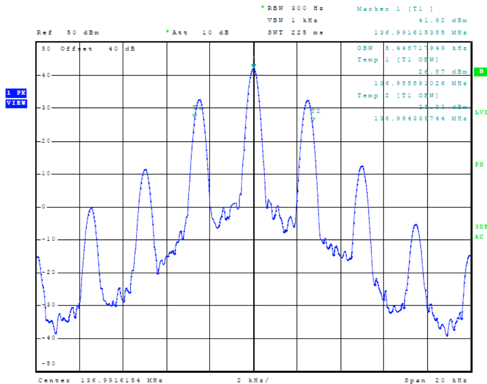
Figure 8 Occupied Band Width Carrier frequency 136.992 MHz
