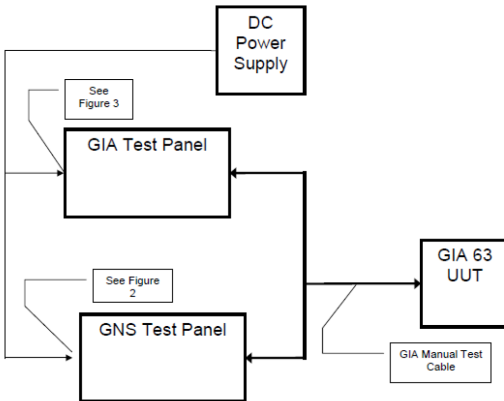
Figure 1: Test Setup Block Diagram
