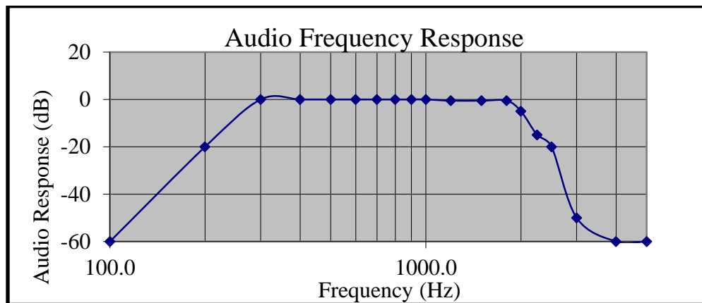
Figure 3 Audio Frequency Response / Modulation Characteristics
