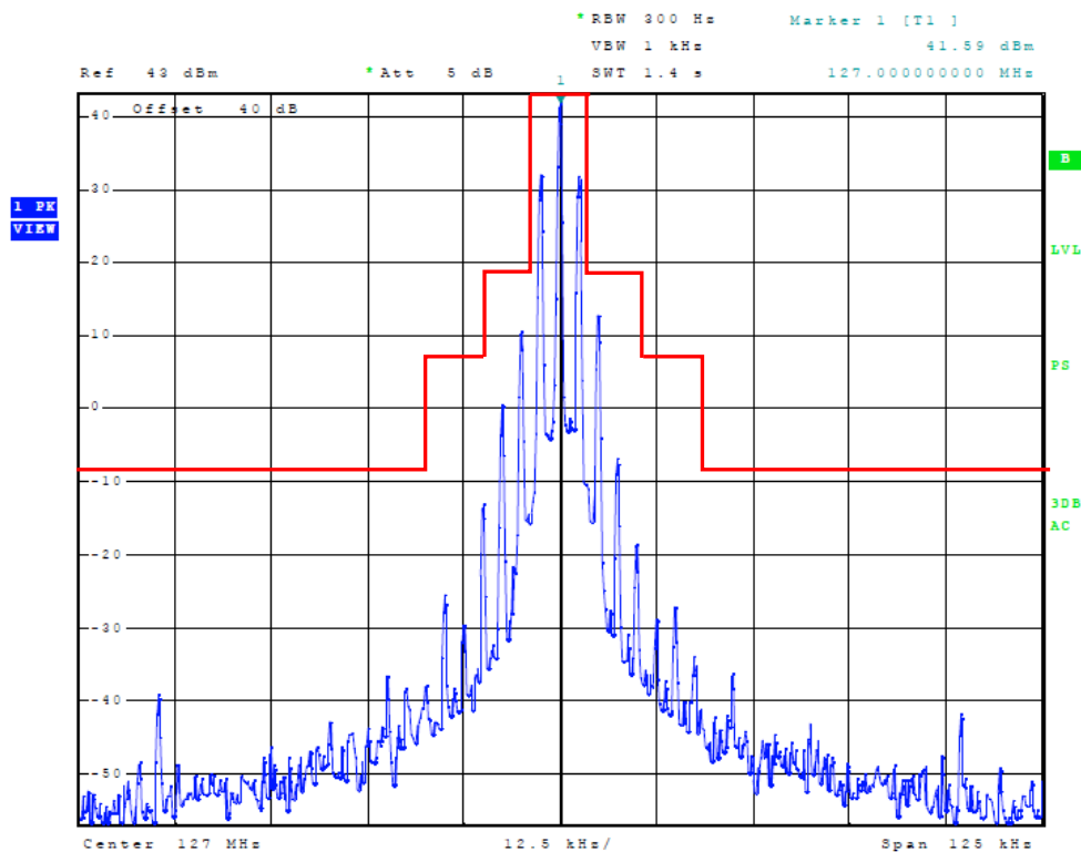
Figure 10 Emission Mask
