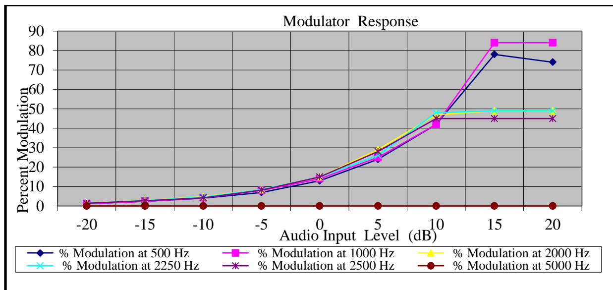
Figure 2 Modulation Characteristics
