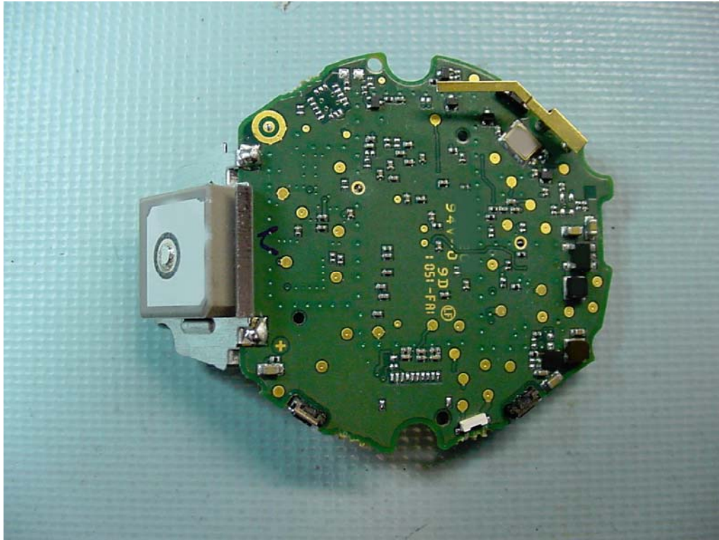
Internal photographs of equipment under test PCB front and Back
