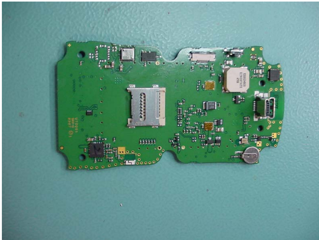
Back PCB
