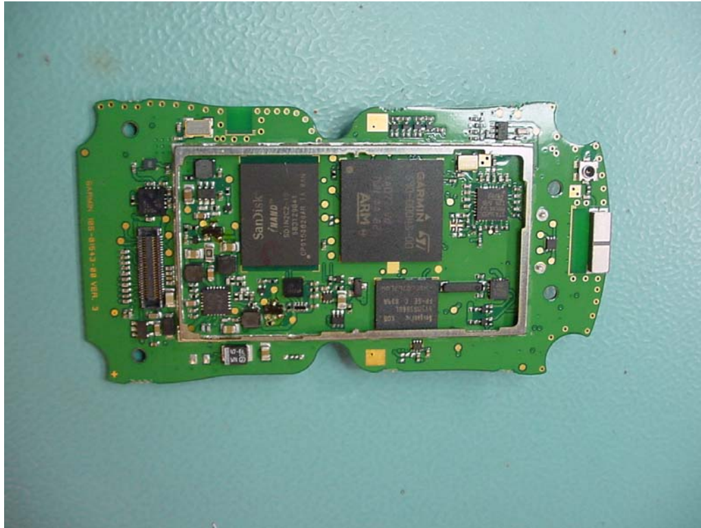
Internal Photographs Front PCB with shield removed
