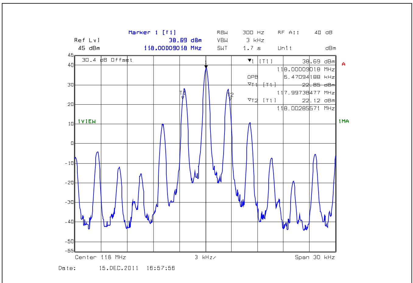
Plot 5.4.4.1.1. Occupied Bandwidth for 118 MHz, 8.33 kHz Channel Spacing
