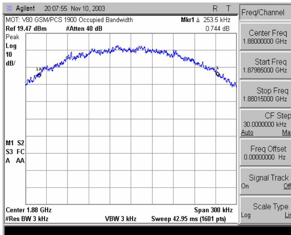
1900 GSM Occupied Bandwidth
