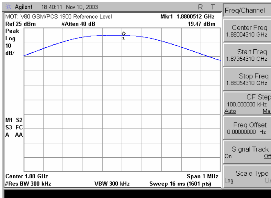
1900 GSM Reference Level
