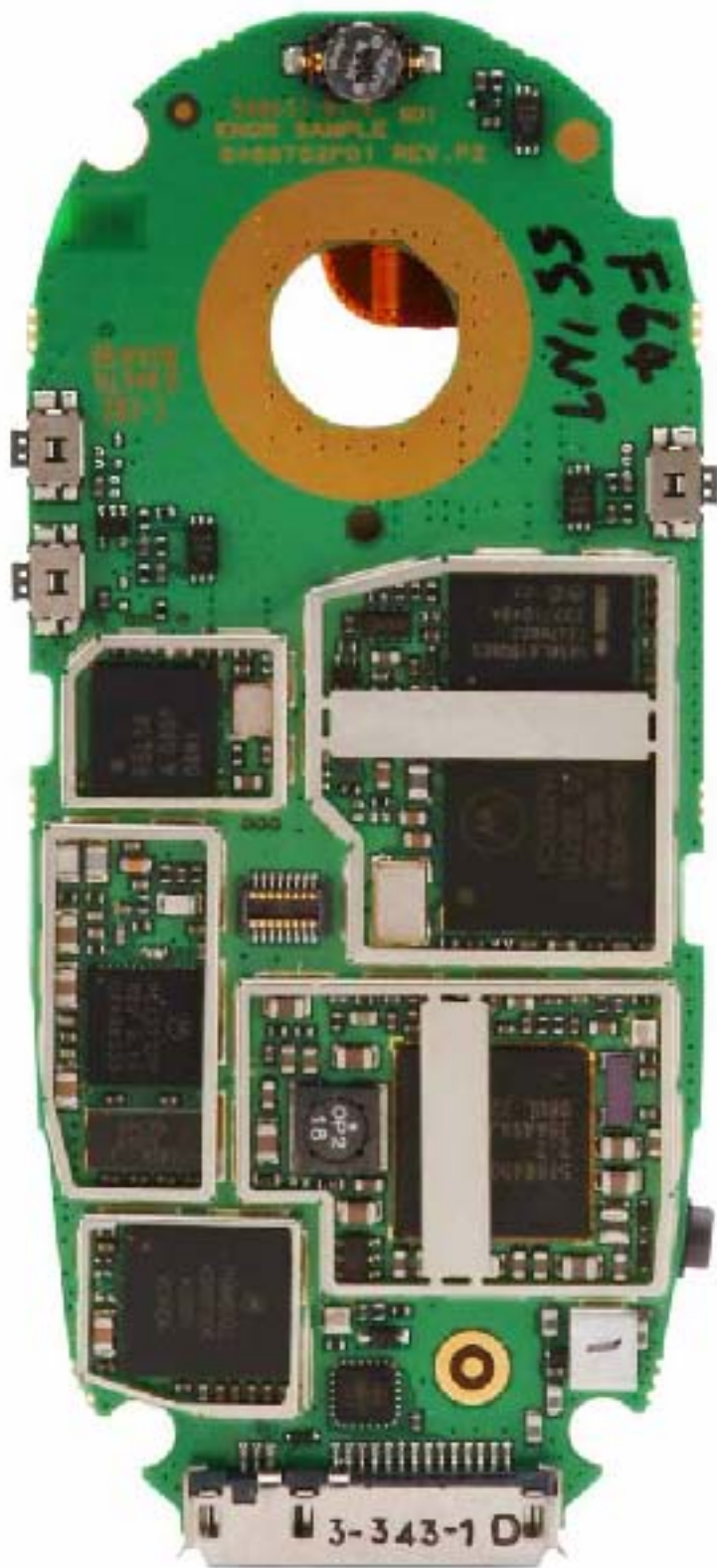
Front View (Shields Removed)
