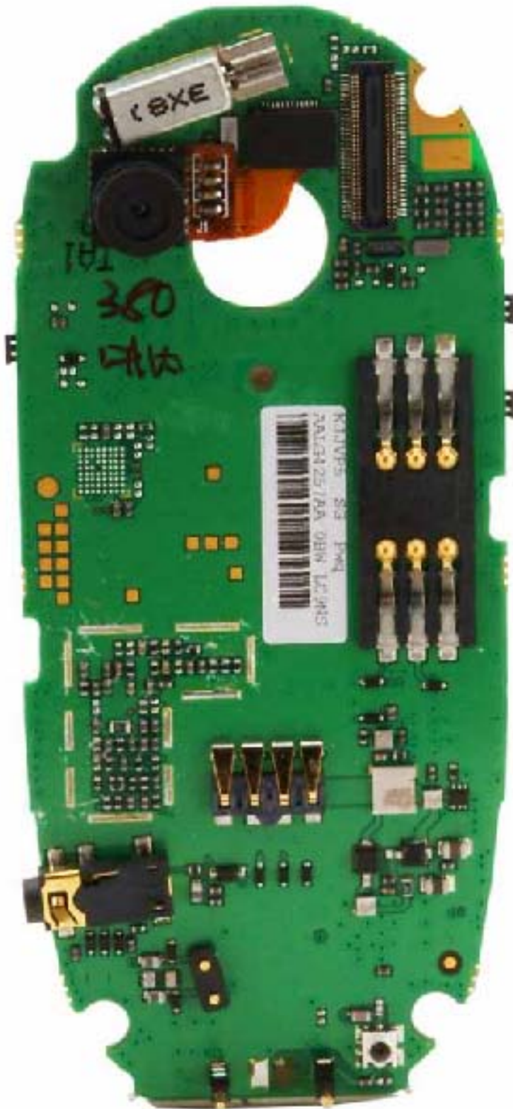
Rear View (Shields Removed)
