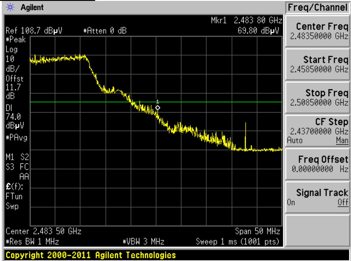
Plot 6-40. Radiated Restricted Upper Band Edge Measurement (Peak)
