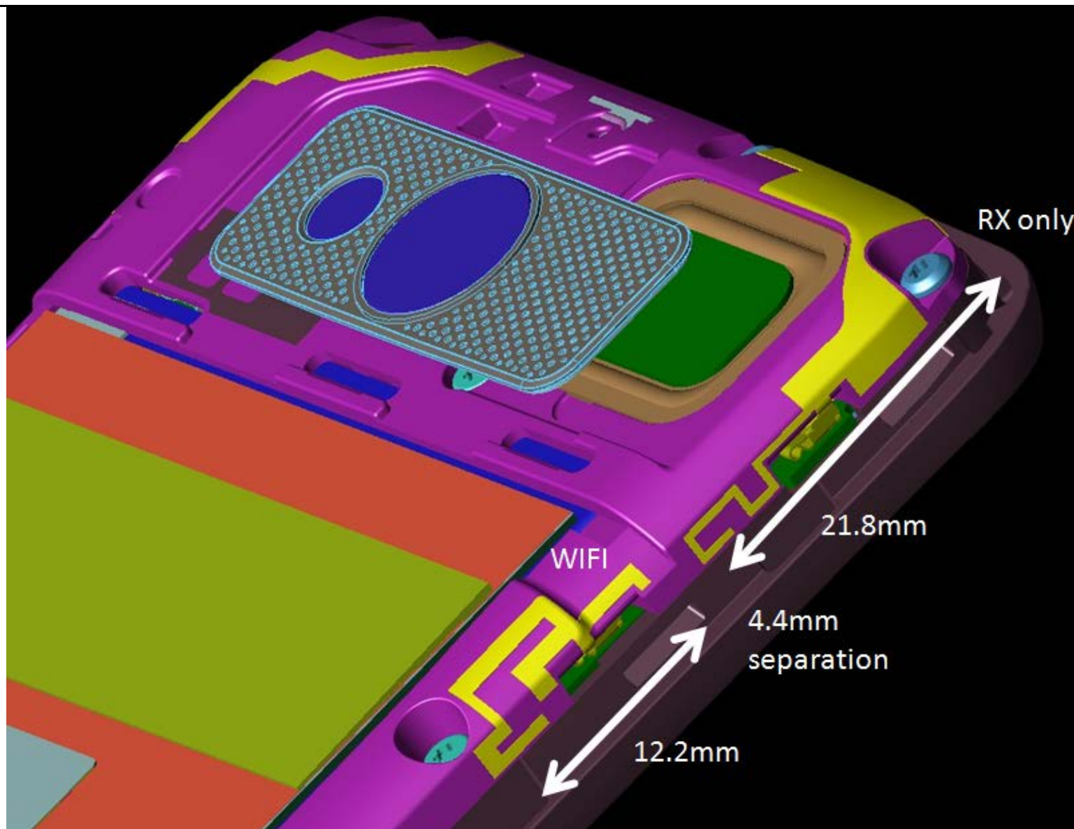
Photograph 9-6: Antenna Spacings.
