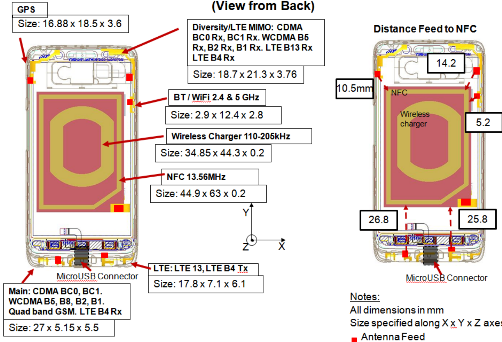
Photograph 9-4: Antenna Locations.
