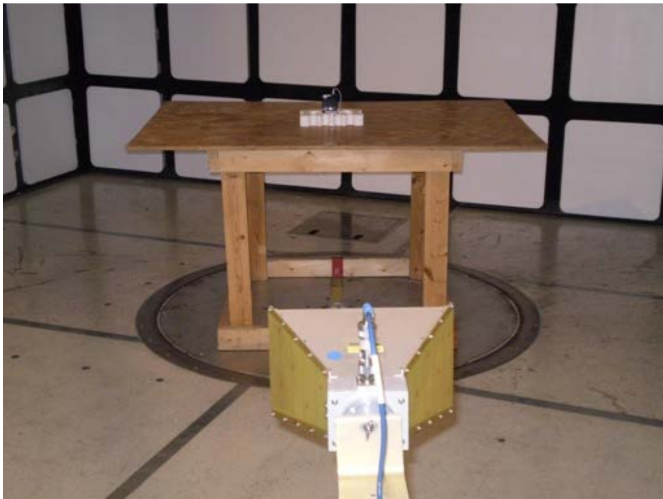
Figure 7c1-2: TX Radiated Configuration.
