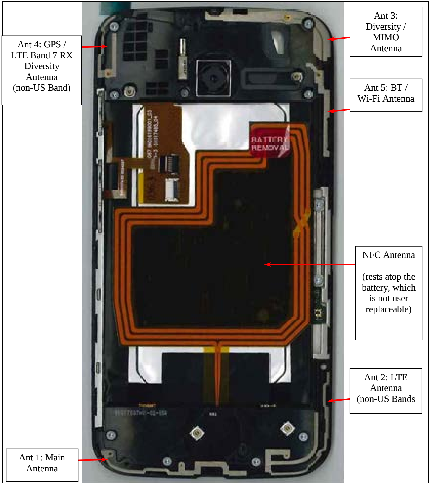
Photograph 9-4: Antenna Locations.
