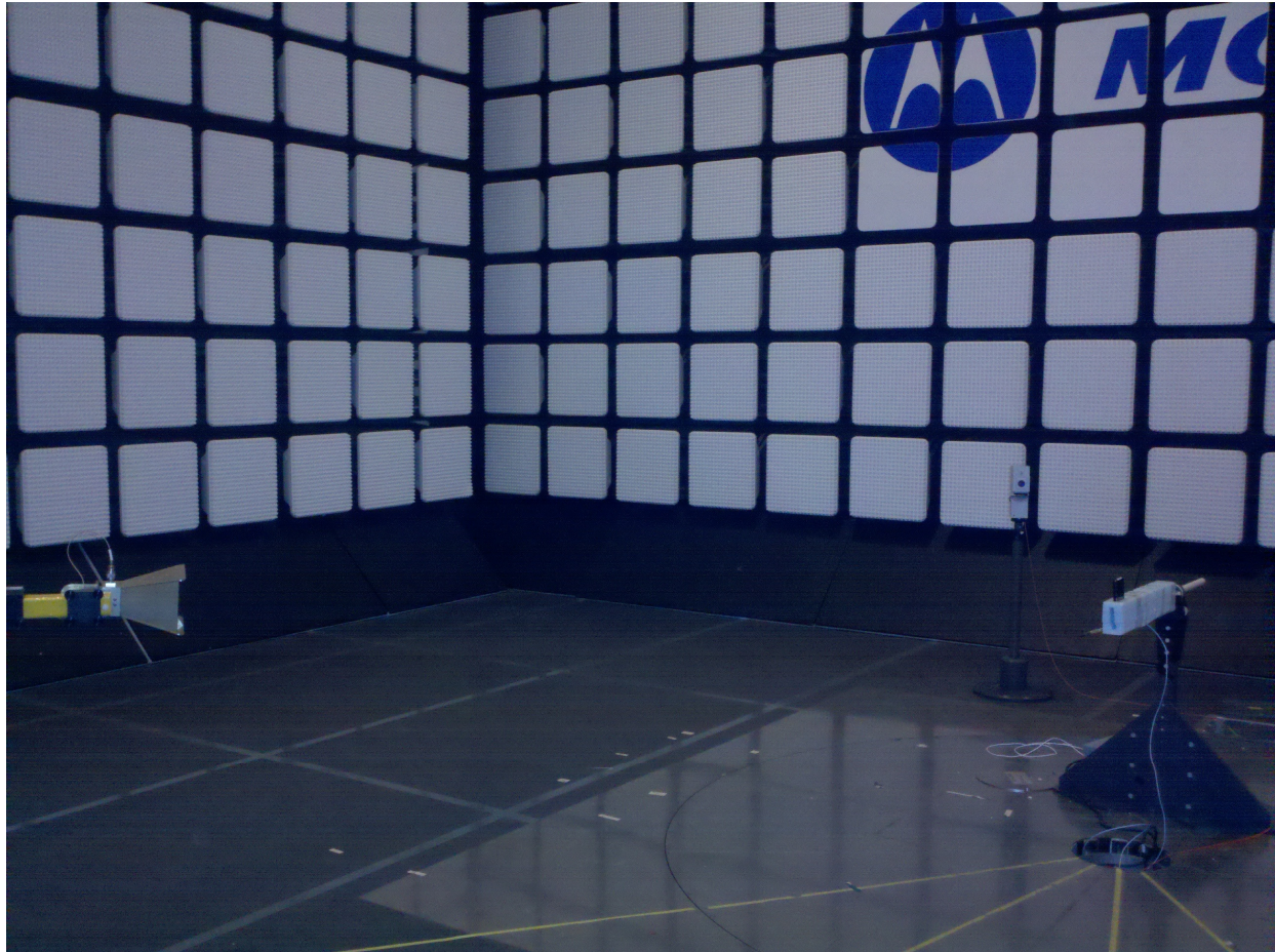
Radiated Emissions
