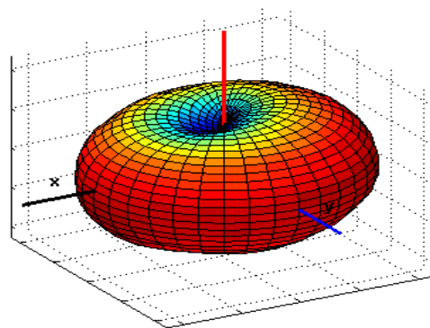
Figure 6a.6-2 Antenna pattern in the 800 MHz band (Flip Closed).
