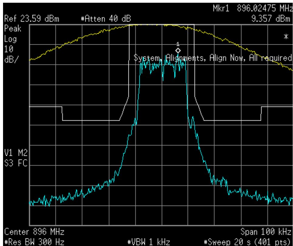
Figure 6a.2.2-3. iDEN 900 MHz Band, Quad-QPSK, Max. Power, EA Emission Mask
