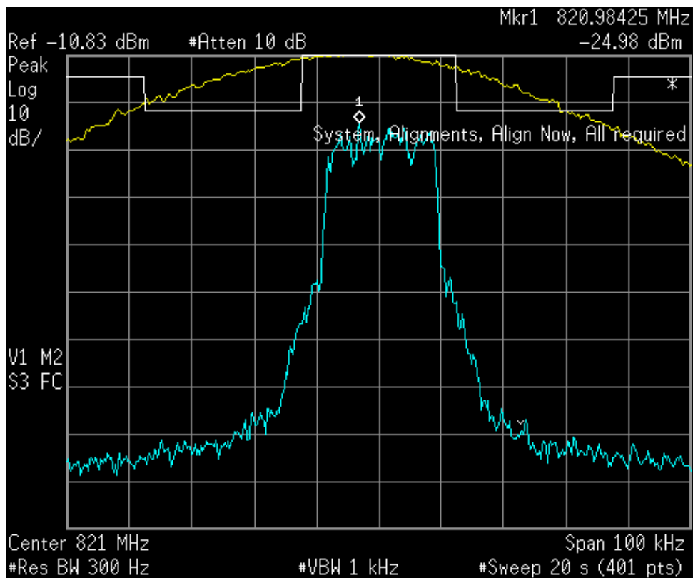
Figure 6a.2.1-8. iDEN 800 MHz Band, Quad-16QAM, Min. Power, EA Emission Mask
