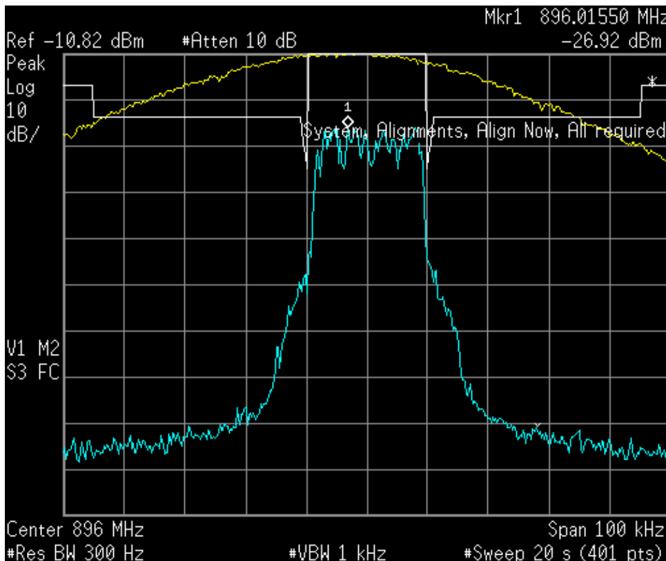
Figure 6a.2.2-6. iDEN 900 MHz Band, Quad-16QAM, Min. Power, Emission Mask G
