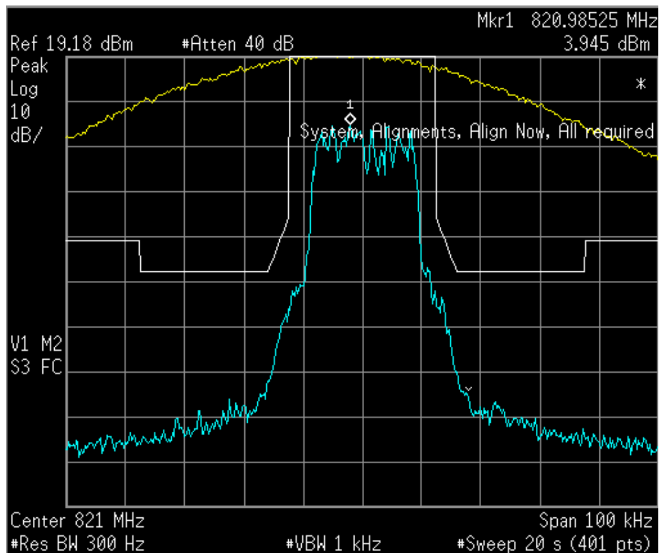
Figure 6a.2.1-7. iDEN 800 MHz Band, Quad-16QAM, Max. Power, EA Emission Mask
