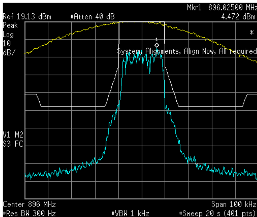
Figure 6a.2.2-1. iDEN 900 MHz Band, Quad-QPSK, Max. Power, Emission Mask G
