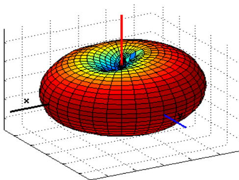
Figure 6a.6-1 Antenna pattern in the 800 MHz band (Flip Open).
