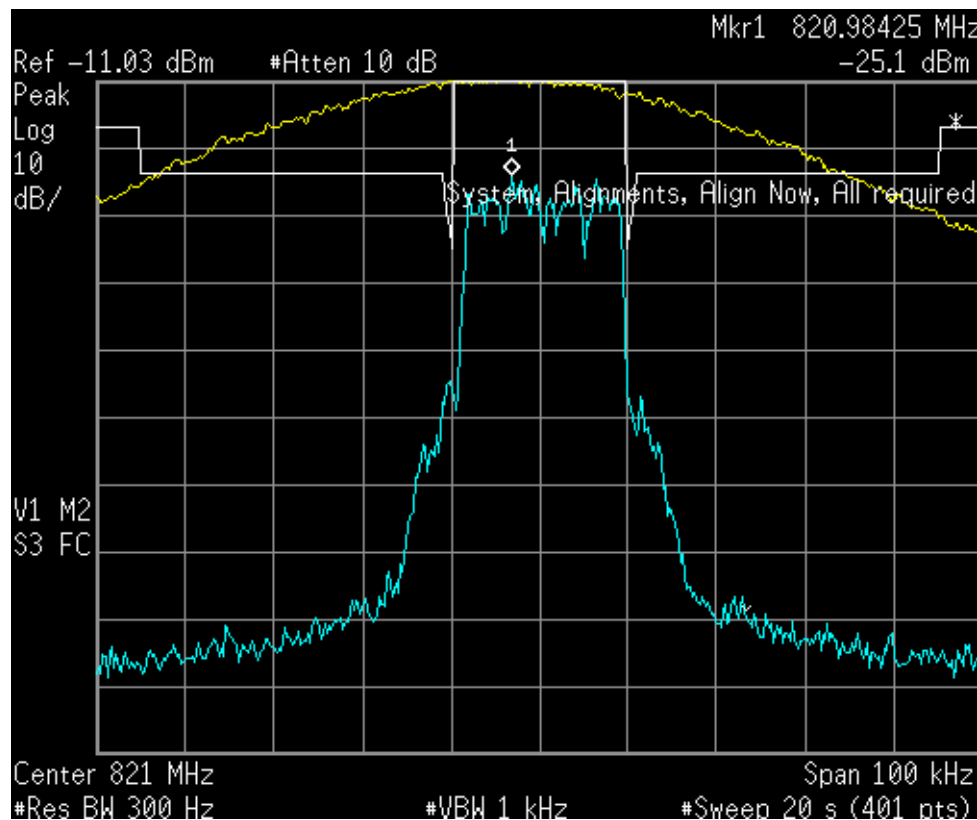
Figure 6a.2.1-6. iDEN 800 MHz Band, Quad-16QAM, Min. Power, Emission Mask G
