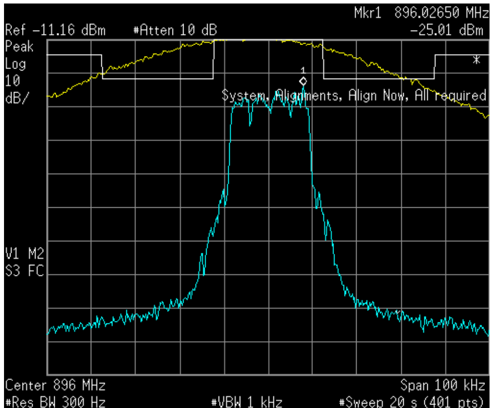
Figure 6a.2.2-8. iDEN 900 MHz Band, Quad-16QAM, Min. Power, EA Emission Mask
