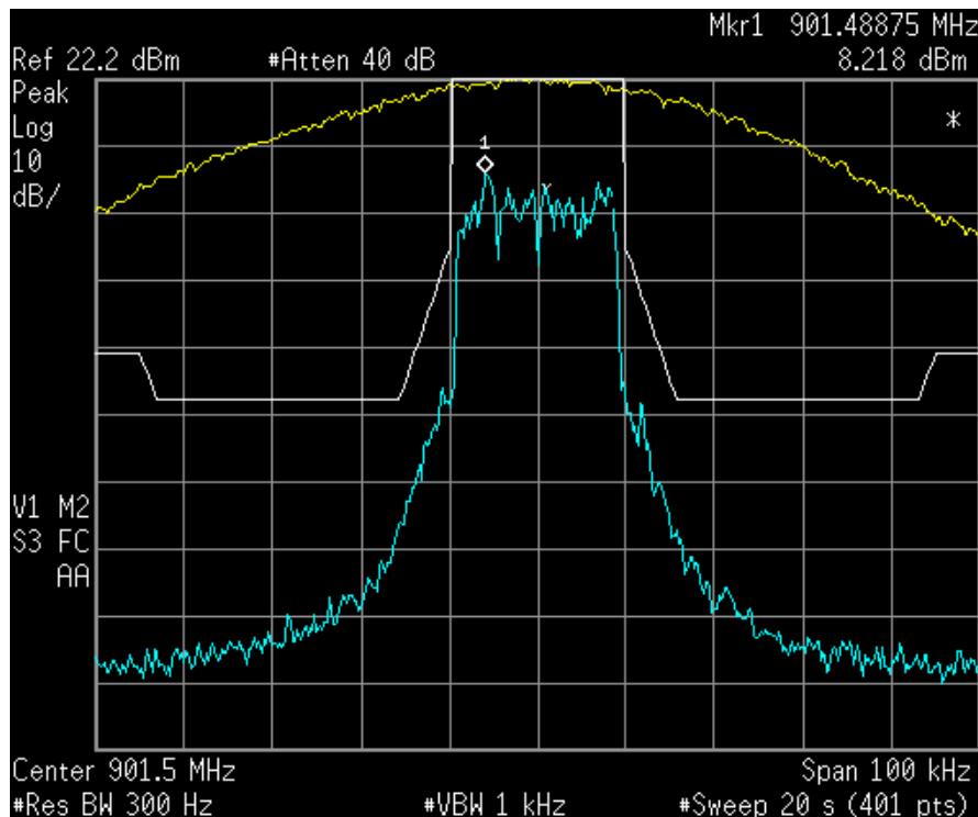
Figure 6b.2.1-1 iDEN NBPCS Band, Occupied Bandwidth, Quad-QPSK, Max. Power.
