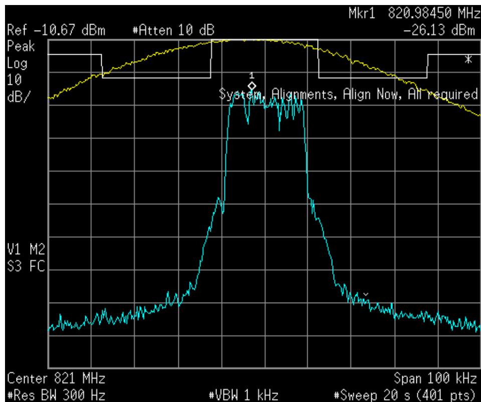
Figure 6a.2.1-12. iDEN 800 MHz Band, Quad-64QAM, Min. Power, EA Emission Mask
