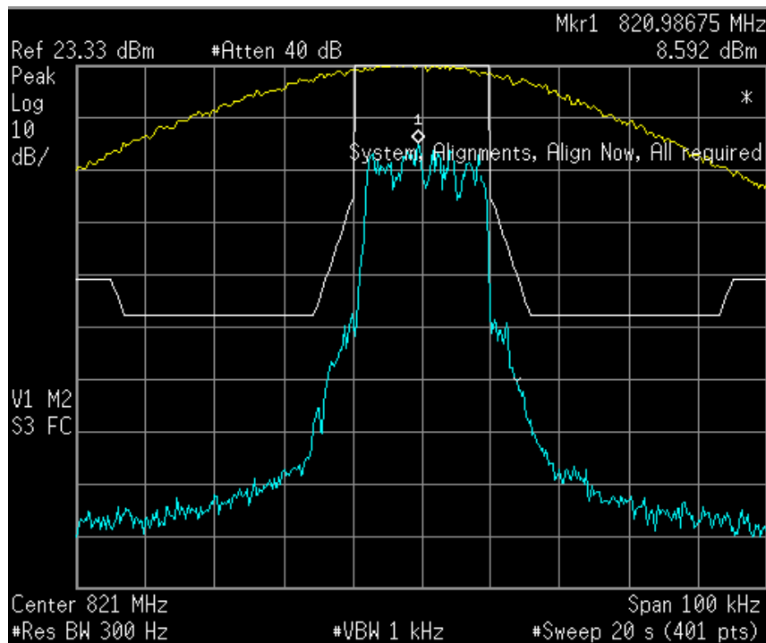
Figure 6a.2.1-1. iDEN 800 MHz Band, Quad-QPSK, Max. Power, Emission Mask G
