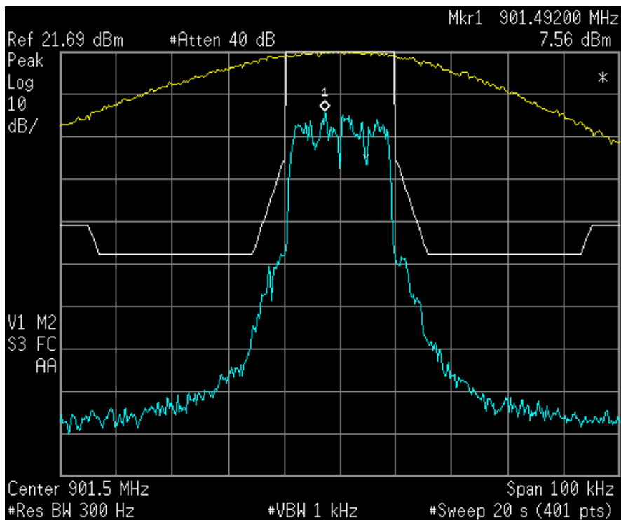
Figure 6b.2.1-2 iDEN NBPCS Band, Occupied Bandwidth, Quad-16QAM, Max. Power.
