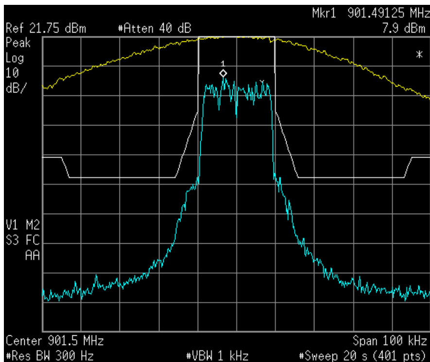
Figure 6b.2.1-3. iDEN NBPCS Band, Occupied Bandwidth, Quad-64QAM, Max. Power.
