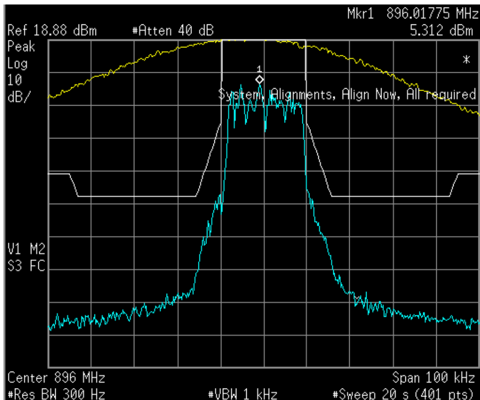
Figure 6a.2.2-5. iDEN 900 MHz Band, Quad-16QAM, Max. Power, Emission Mask G
