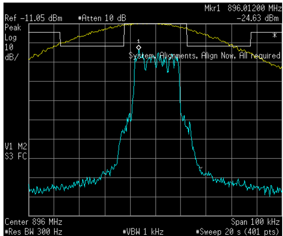
Figure 6a.2.2-12. iDEN 900 MHz Band, Quad-64QAM, Min. Power, EA Emission Mask
