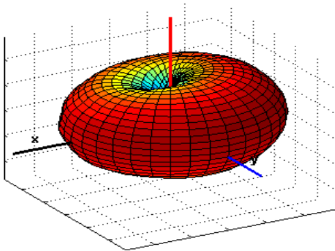
Figure 6a.6-3 Antenna pattern in the 900 MHz band (Flip Open).
