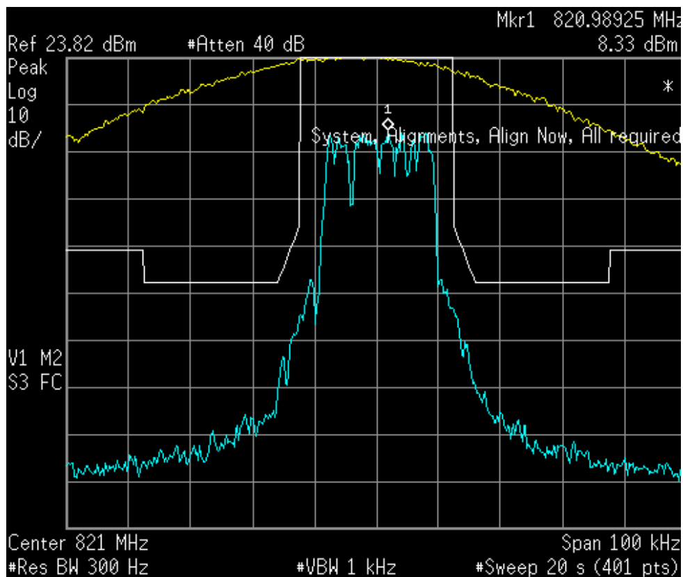
Figure 6a.2.1-11. iDEN 800 MHz Band, Quad-64QAM, Max. Power, EA Emission Mask
