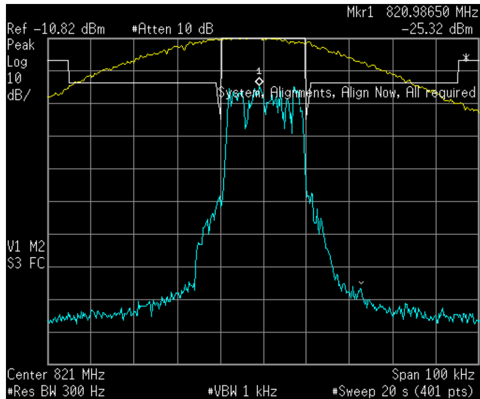
Figure 6a.2.1-10. iDEN 800 MHz Band, Quad-64QAM, Min. Power, Emission Mask G
