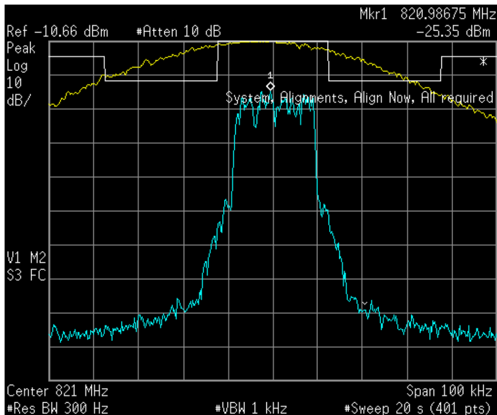
Figure 6a.2.1-4. iDEN 800 MHz Band, Quad-QPSK, Min.m Power, EA Emission Mask
