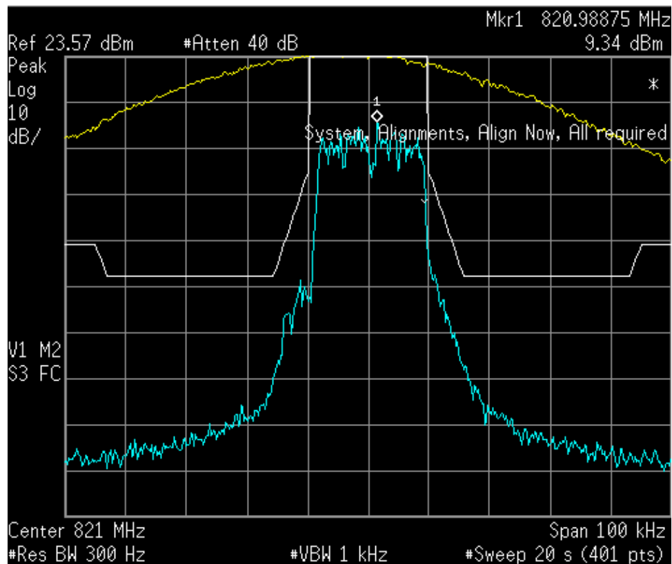
Figure 6a.2.1-9. iDEN 800 MHz Band, Quad-64QAM, Max. Power, Emission Mask G
