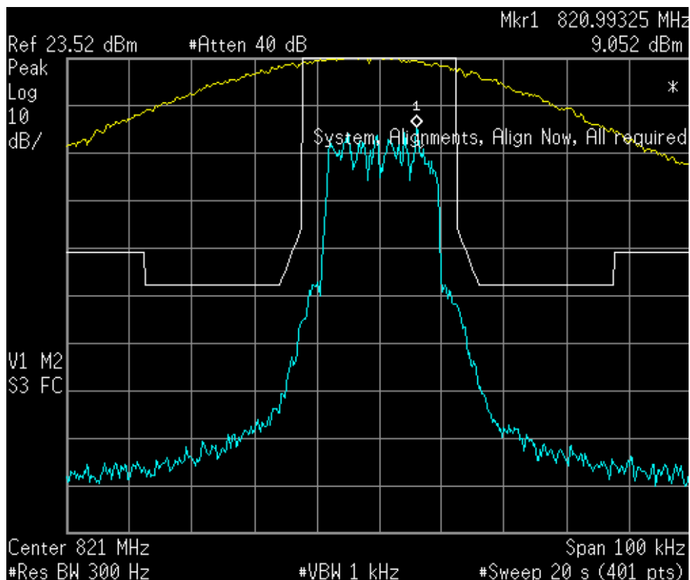
Figure 6a.2.1-3. iDEN 800 MHz Band, Quad-QPSK, Max. Power, EA Emission Mask
