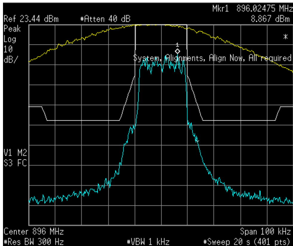
Figure 6a.2.2-9. iDEN 900 MHz Band, Quad-64QAM, Max. Power, Emission Mask G
