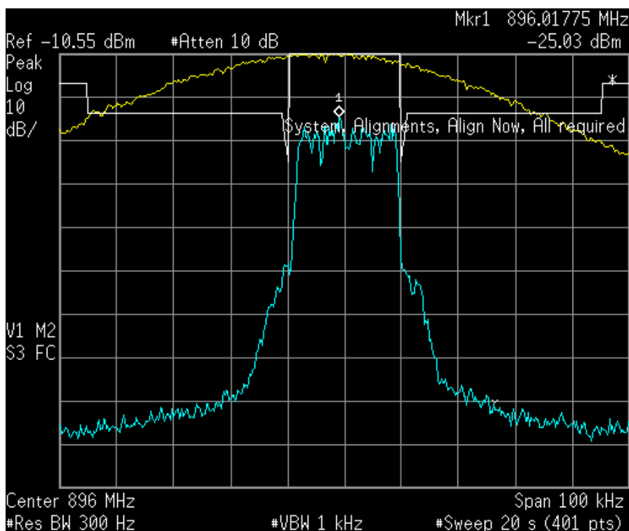
Figure 6a.2.2-2. iDEN 900 MHz Band, Quad-QPSK, Min. Power, Emission Mask G
