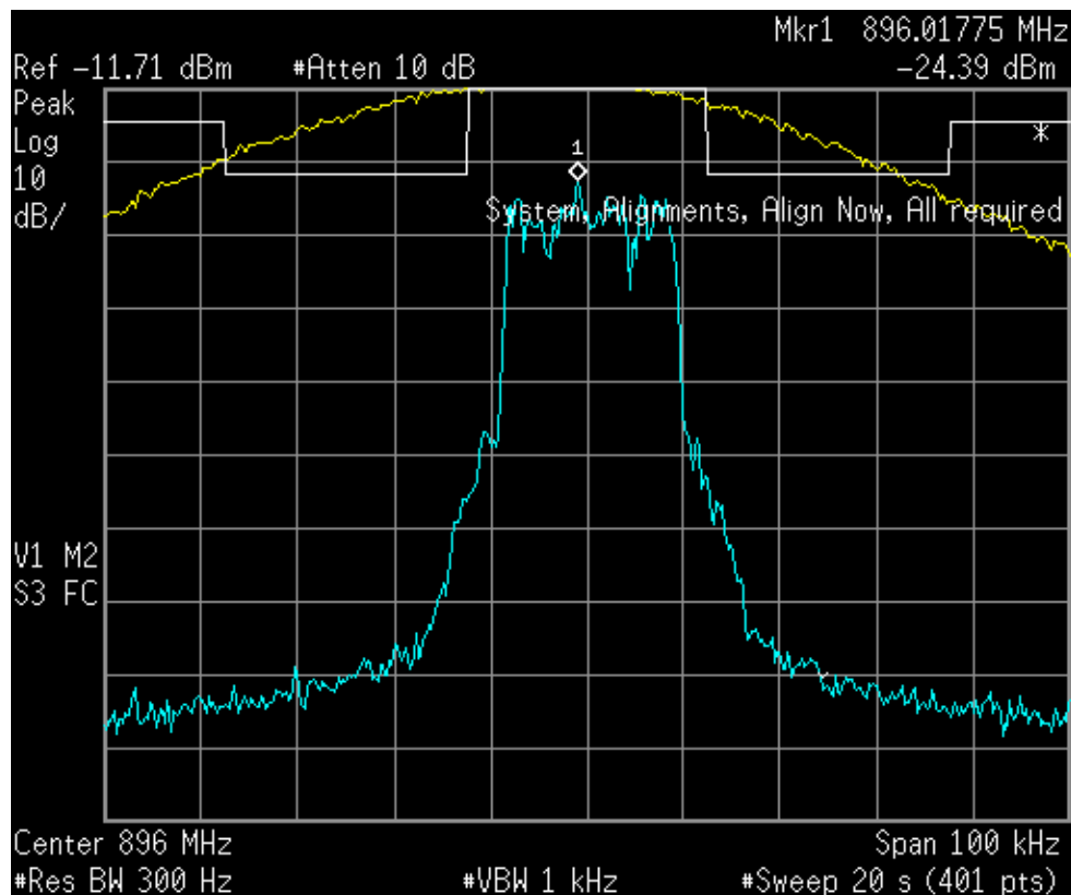
Figure 6a.2.2-4. iDEN 900 MHz Band, Quad-QPSK, Min. Power, EA Emission Mask
