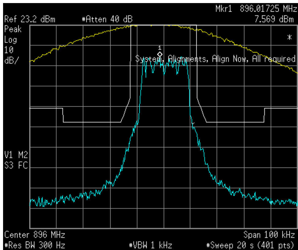
Figure 6a.2.2-11. iDEN 900 MHz Band, Quad-64QAM, Max. Power, EA Emission Mask
