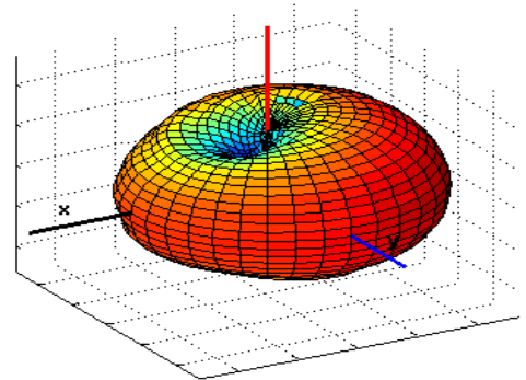
Figure 6a.6-4 Antenna pattern in the 900 MHz band (Flip Closed).
