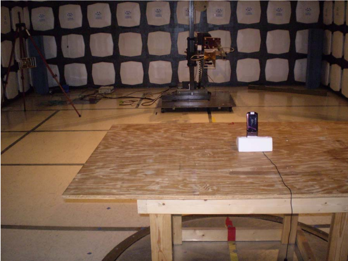
EMC Report #20499-1, Tx Radiated
