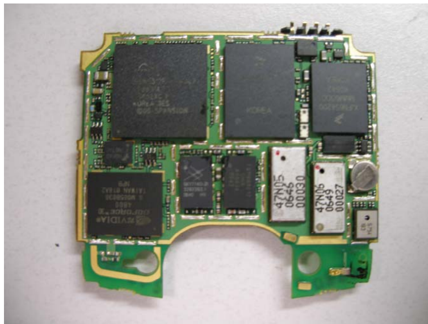
Main Board Top Without Popples
