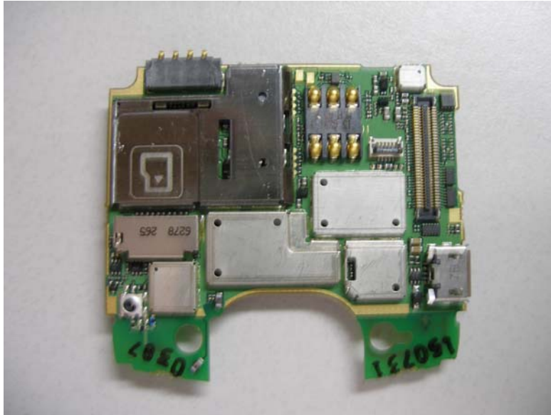
Main Board Bottom With Shields
