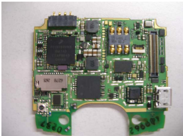
Main Board Bottom Without Shields
