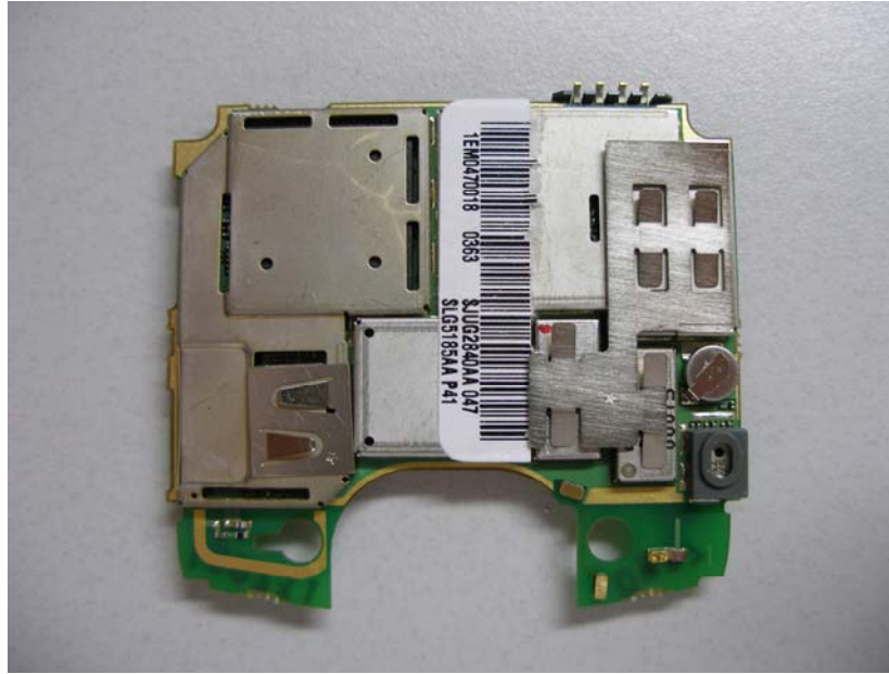
Main Board Top With Shields
