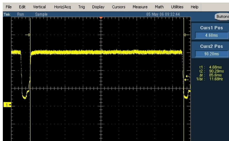
Figure 6c-2.5.1. MOTotalk ISM Band Average Measured Time of Occupancy.
