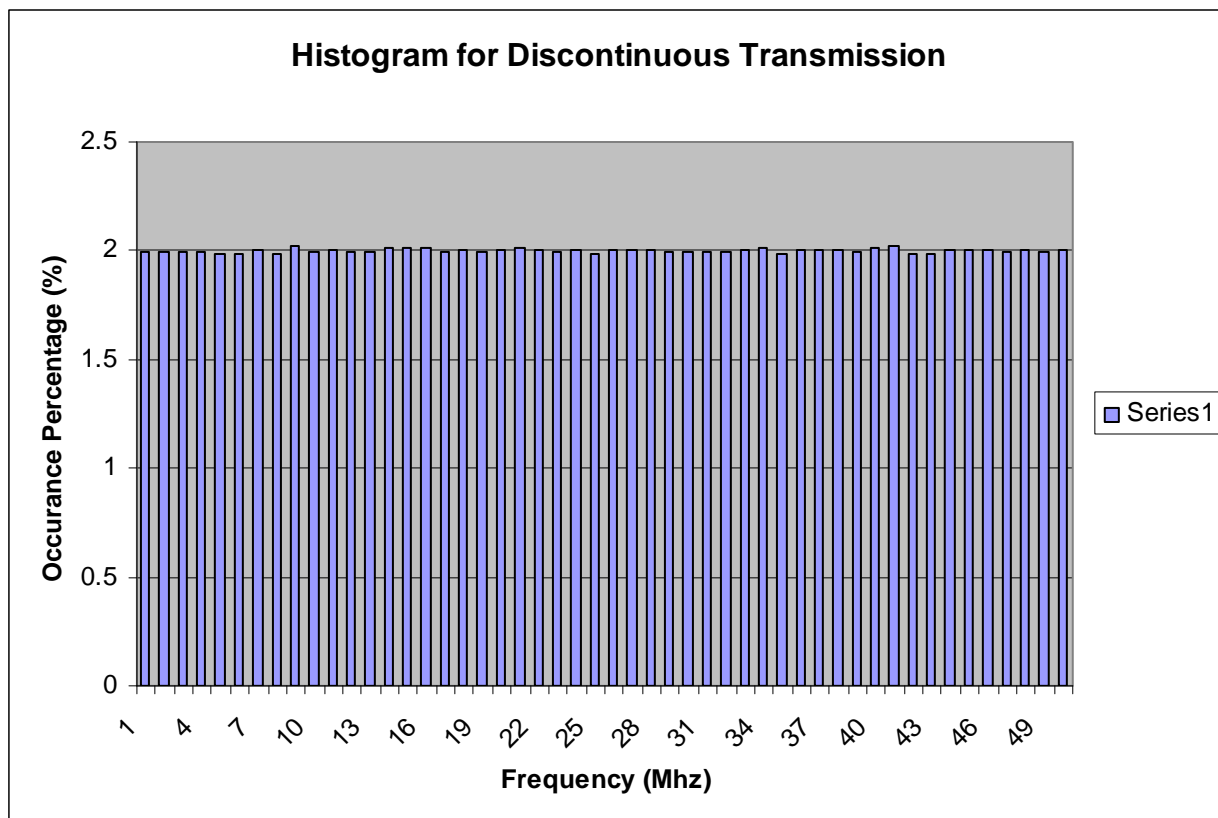
Figure 6c-2.7.1. Histogram for MOTotalk ISM Band Discontinuous Transmission
