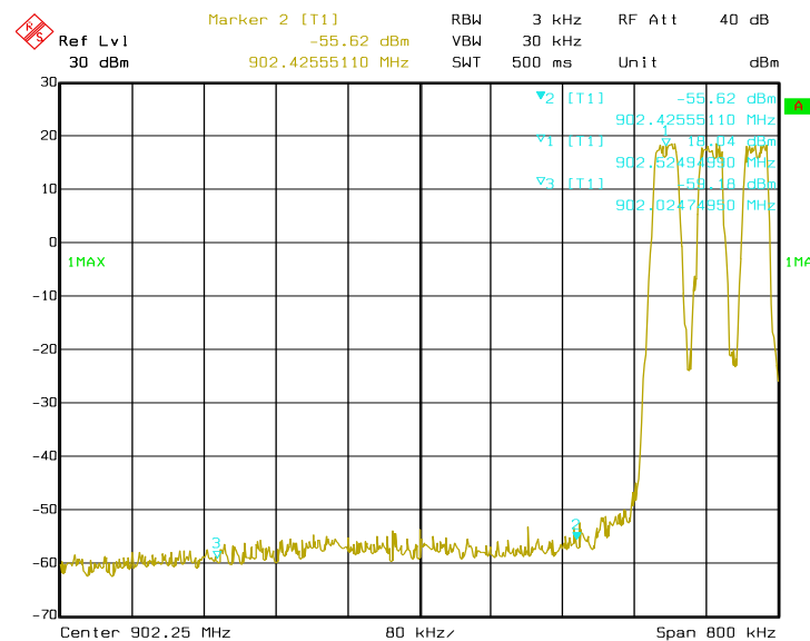
Figure 6c-2.2.4. Out-of-band transmitter spurious emissions low band edge, with hopping function enabled.
