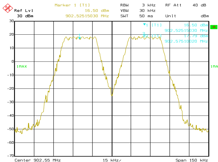
Figure 6c-2.2.2. Adjacent hop set separation with spectrum analyzer center frequency at 902.55 MHz.
