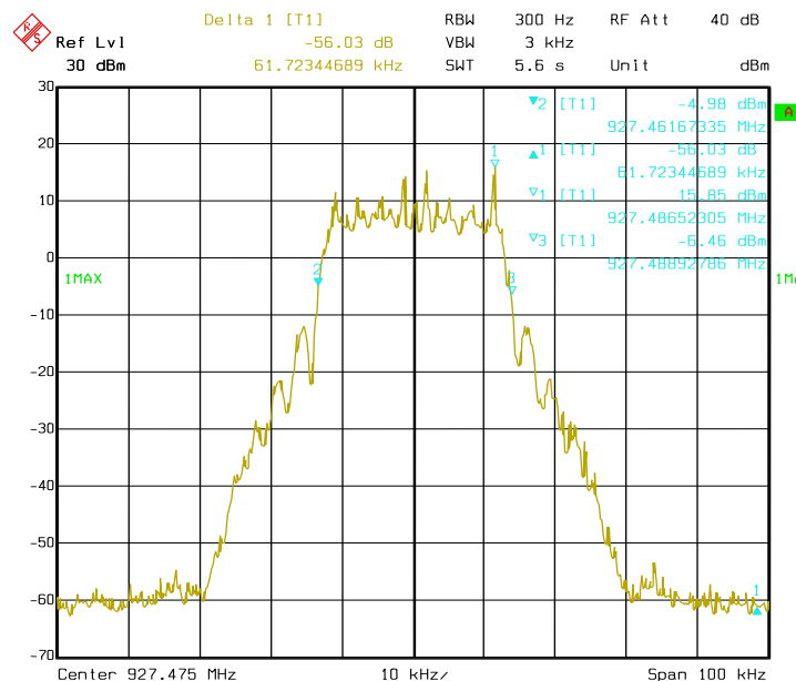
Figure 6c-2.2.5 Spectrum analyzer plot of MOTOtalk ISM Band 8-FSK traffic channel signal's 99% bandwidth with hopping function disabled, at center frequency 927.475 MHz.
