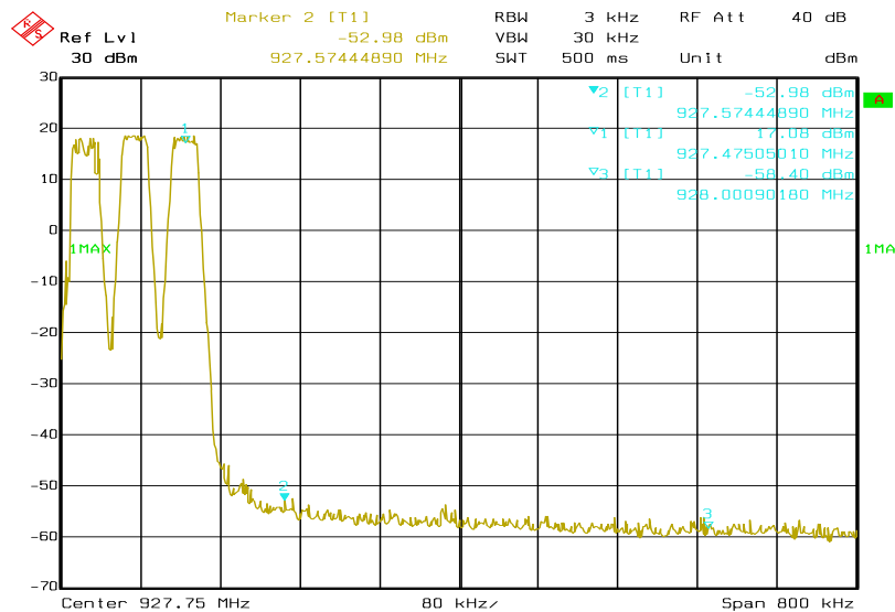
Figure 6c-2.2.8. Out-of-band transmitter spurious emissions high band edge, with hopping function enabled.
