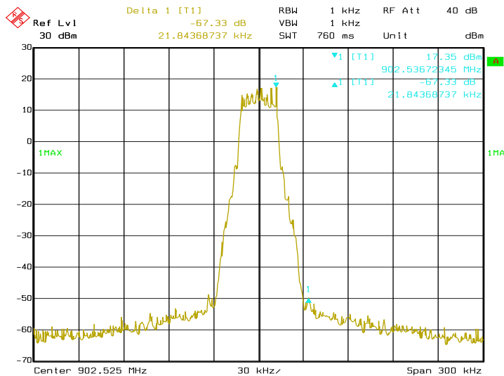
Figure 6c-2.2.3 MOTOTalk ISM band occupied bandwidth with frequency span of 300 kHz with hopping function disabled at center frequency 902.525 MHz.
