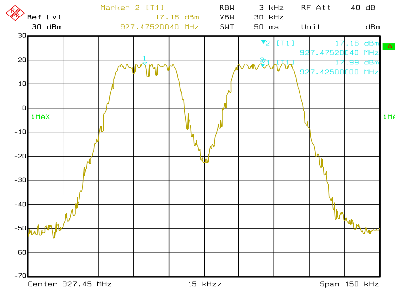
Figure 6c-2.2.6. Adjacent hop set separation with spectrum analyzer center frequency 927.5 MHz.
