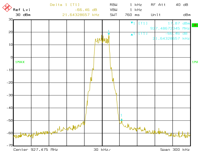
Figure 6c-2.2.7 MOTotalk ISM band occupied bandwidth with frequency span of 300 kHz with hopping function disabled, at center frequency 927.475.
