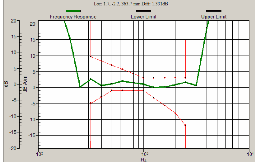
Graph 3: CDMA 1900 Frequency Response with Battery 2
