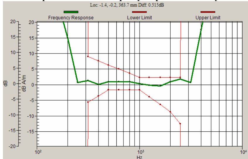
Graph 4: CDMA 1900 Frequency Response with Battery 3
