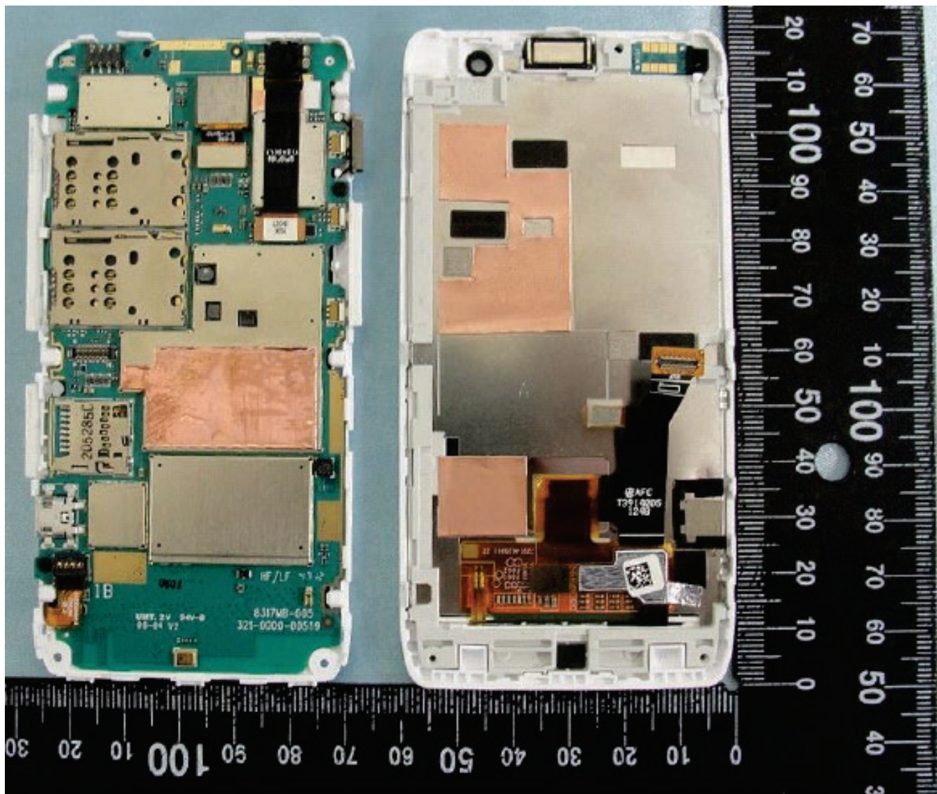
Photograph 9-3: Interior Housing View – PC Board with Shields in Place.
