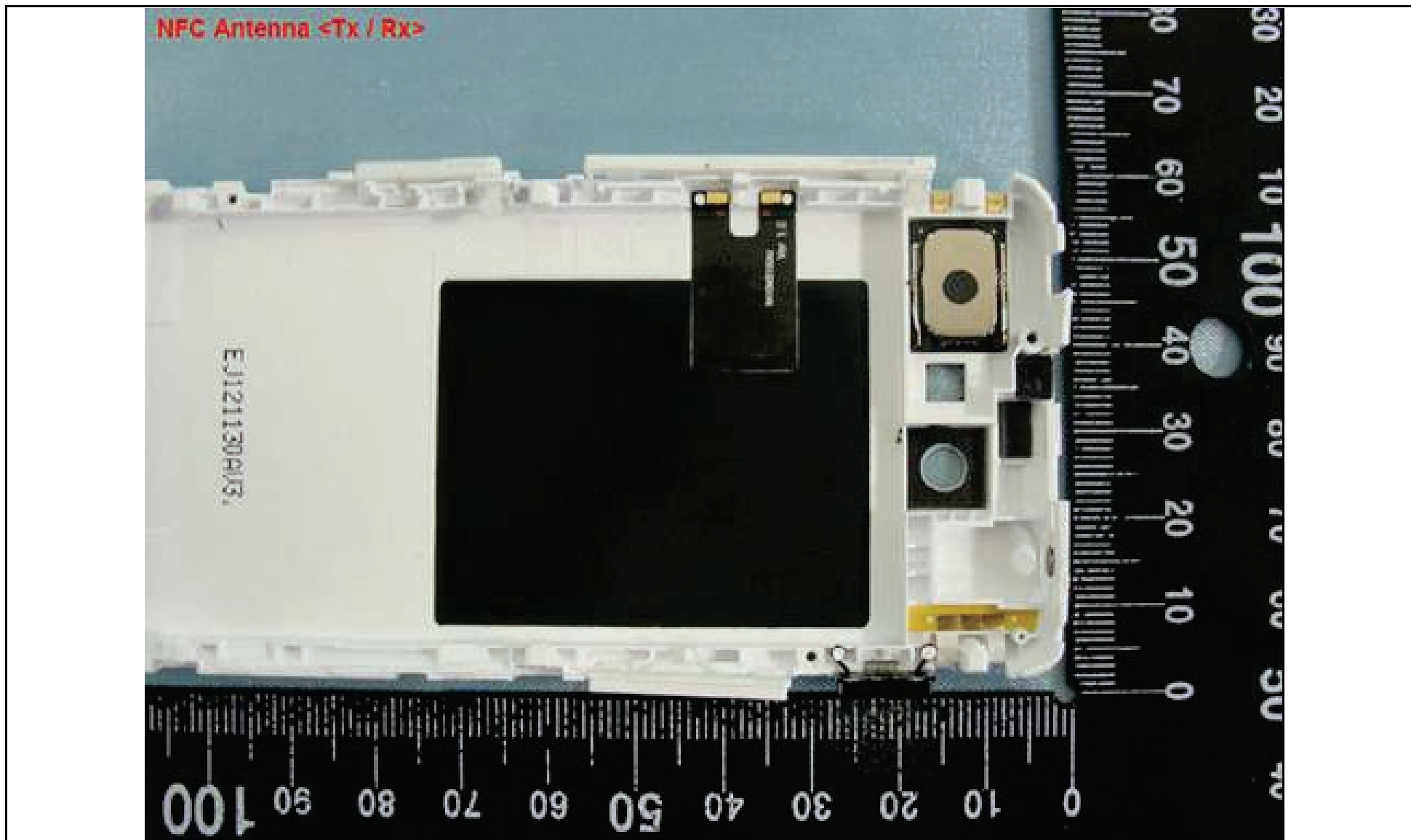
Photograph 9-6: NFC Antenna Detail.
