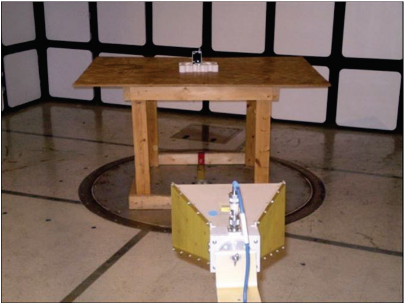
Figure 7B1-1: TX Radiated Configuration.
