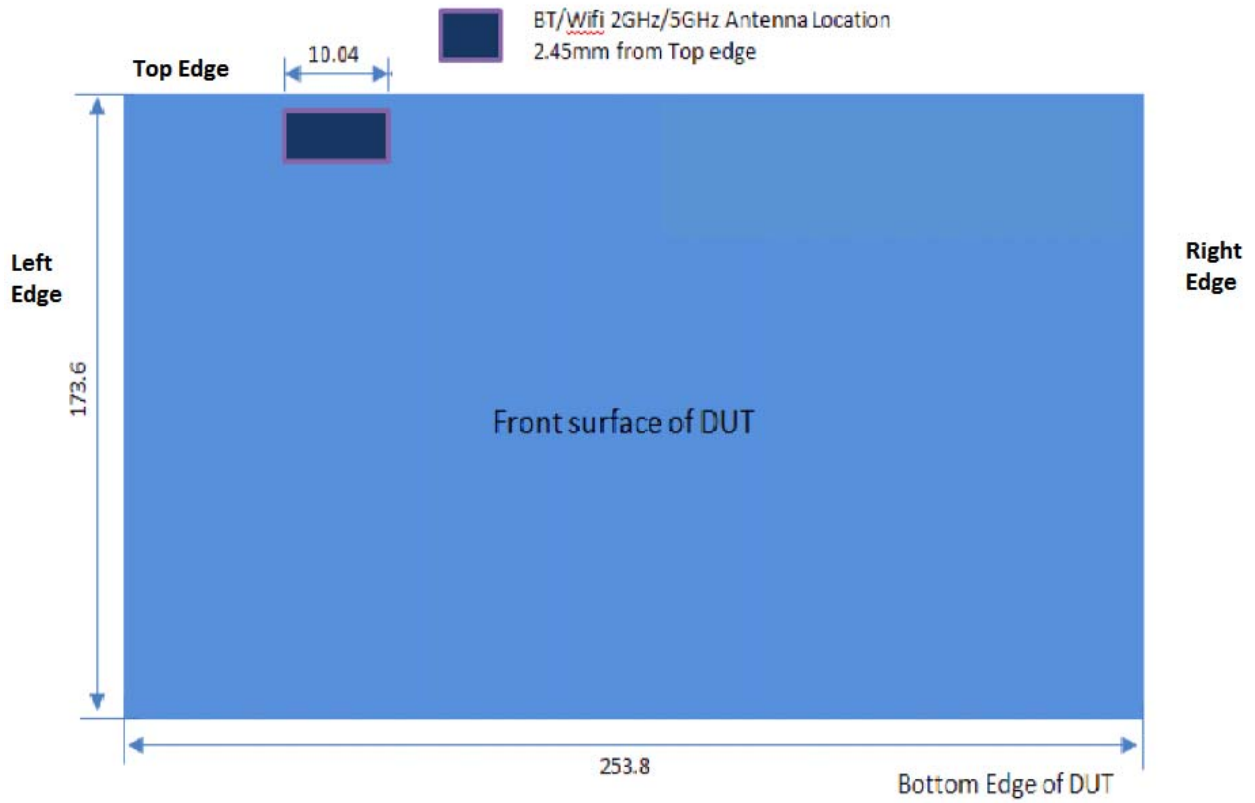
Figure 3: Device Dimensions and Antenna Separation Distances
