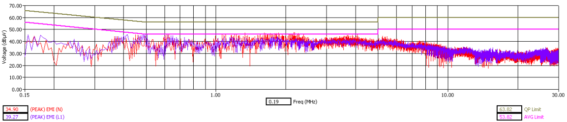
WLAN Channel 48 - Tx Mode - Peak Detector
