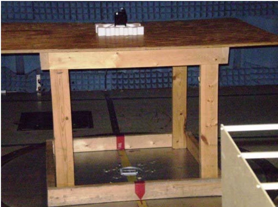
Radiated Emissions
