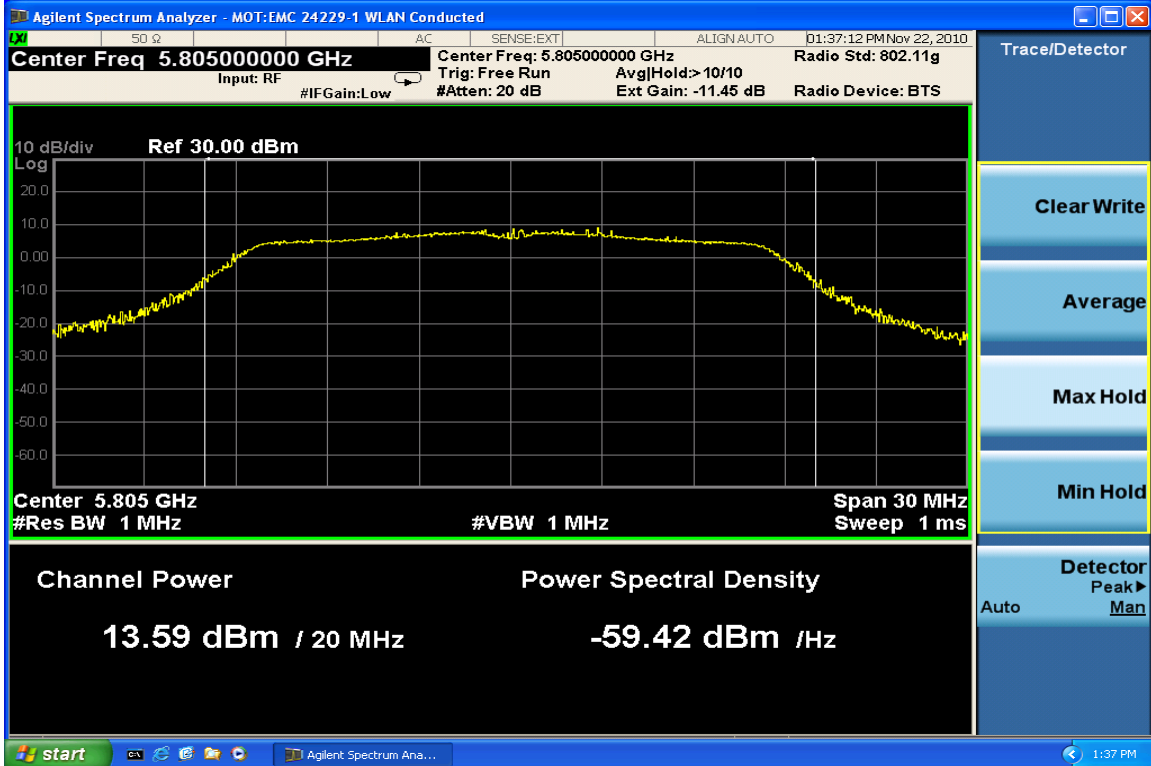
Max. Power Channel 161 @ 6.5 Mbps
