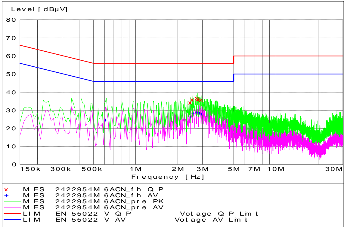
WLAN Channel 157 - Tx Mode - Neutral Coupling
