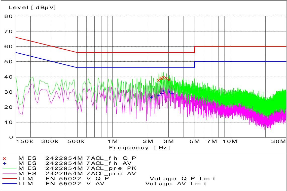
WLAN Channel 157 - Tx Mode - Line Coupling
