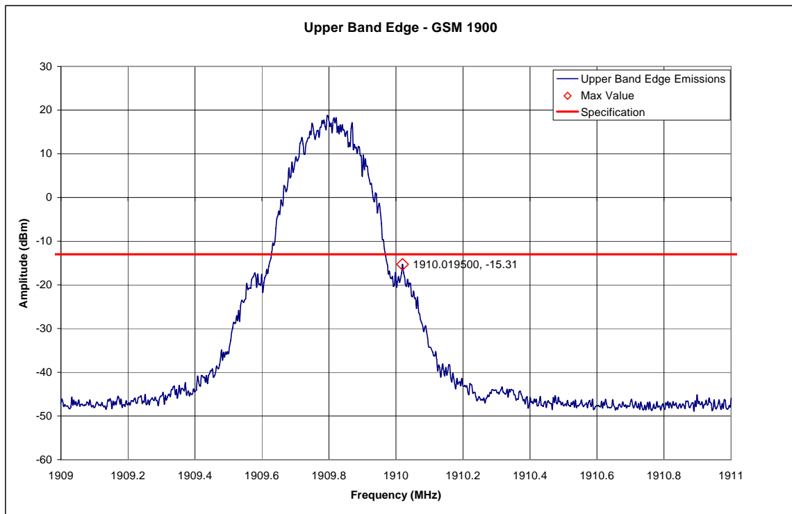
GSM 1900 – Upper Band Edge – Channel 810 (1909.8MHz)
