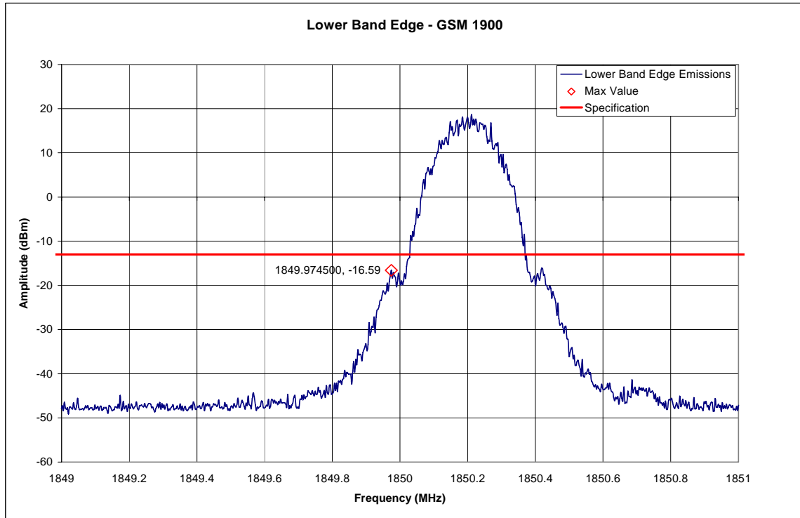
GSM 1900 – Lower Band Edge – Channel 512 (1850.2MHz)
