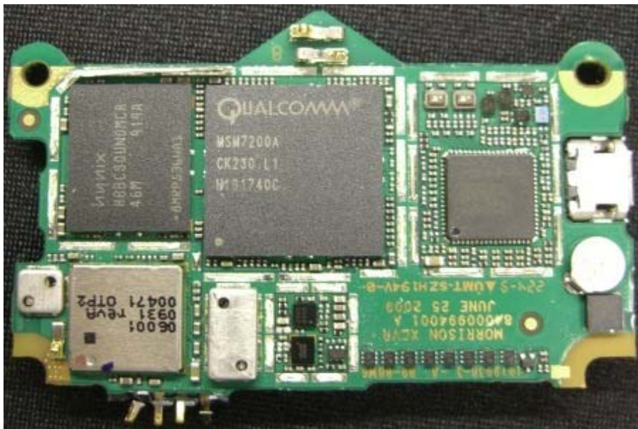
Main PCB Top Side
