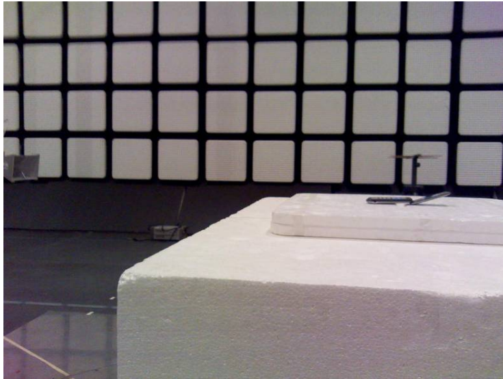
23113-1, IHDP56KP1 setup in semi-anechoic chamber – right view (18 GHz – 26.5 GHz)
