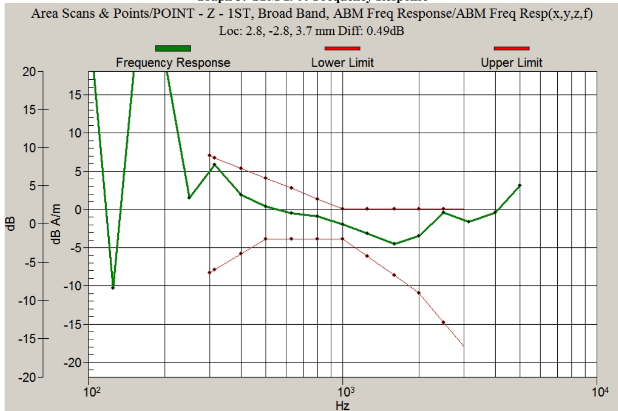
Graph 3: GSM 1900 Frequency Response
