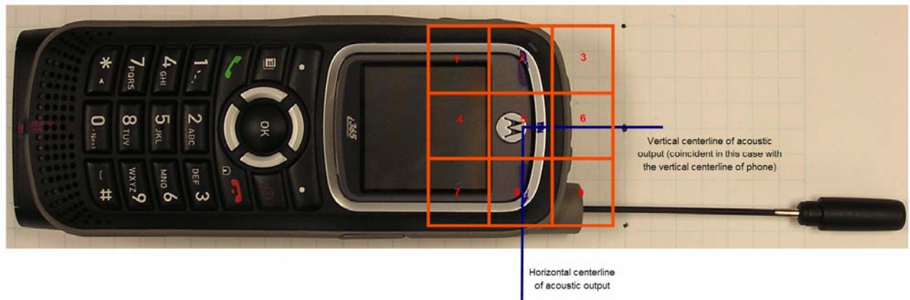
Figure 3. Phone Front - Orientation and Measurement Plane for RF Emissions Testing
