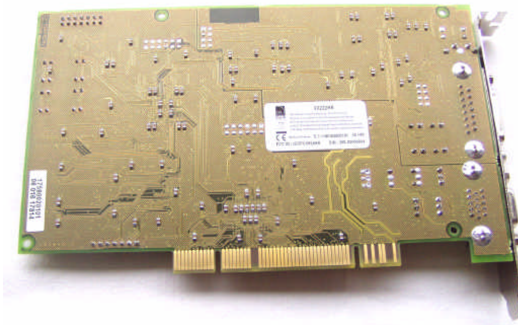
soldering side
