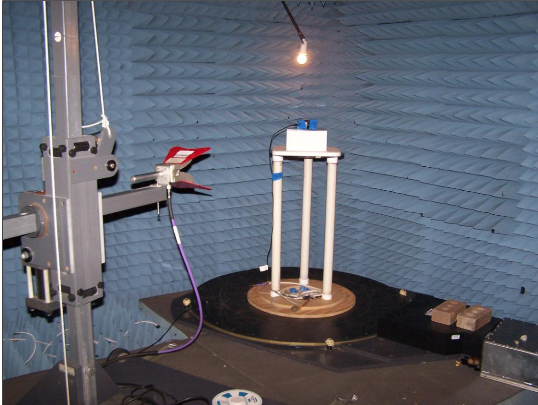
Photograph 1. Radiated Spurious Emissions above 1 GHz, Test Setup
