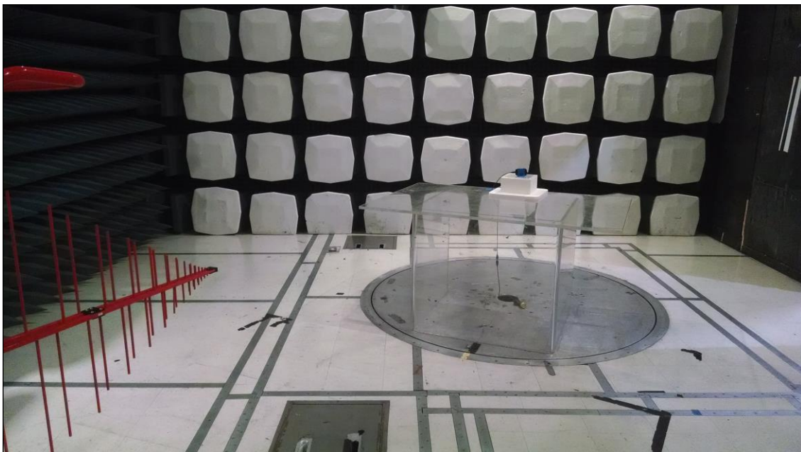
Photograph 2. Radiated Spurious Emissions below 1 GHz, Test Setup
