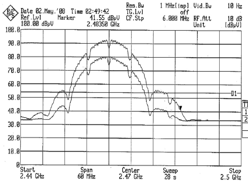
Plot 17 – Average Plot at Upper Band Edge at 2.4835GHz
