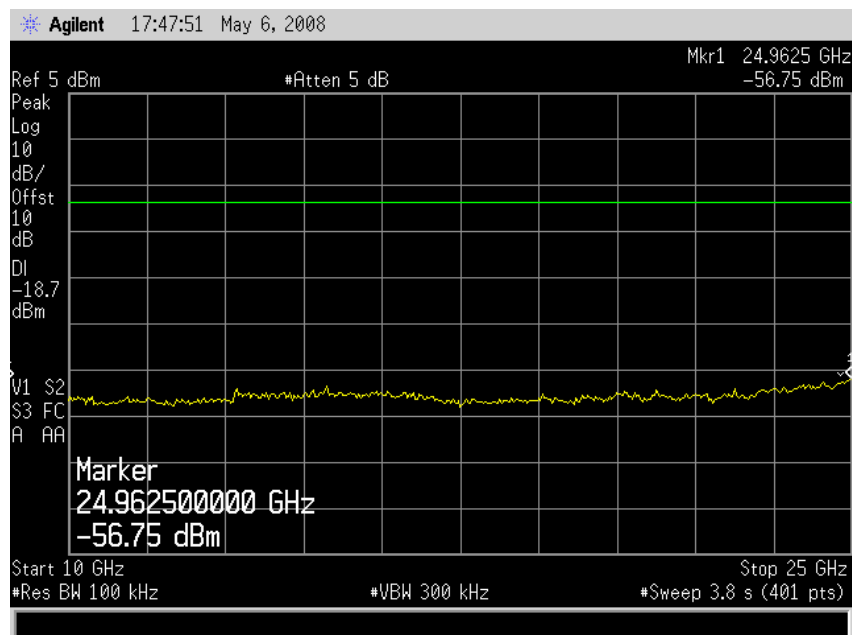
Plot 9 – Channel 2
