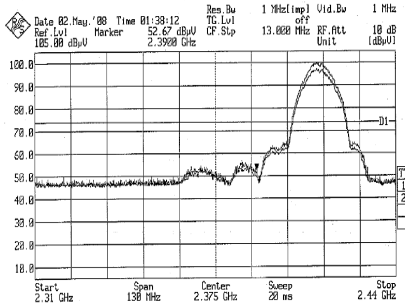
Plot 14 – Peak Plot at Lower Band Edge at 2.4000GHz
