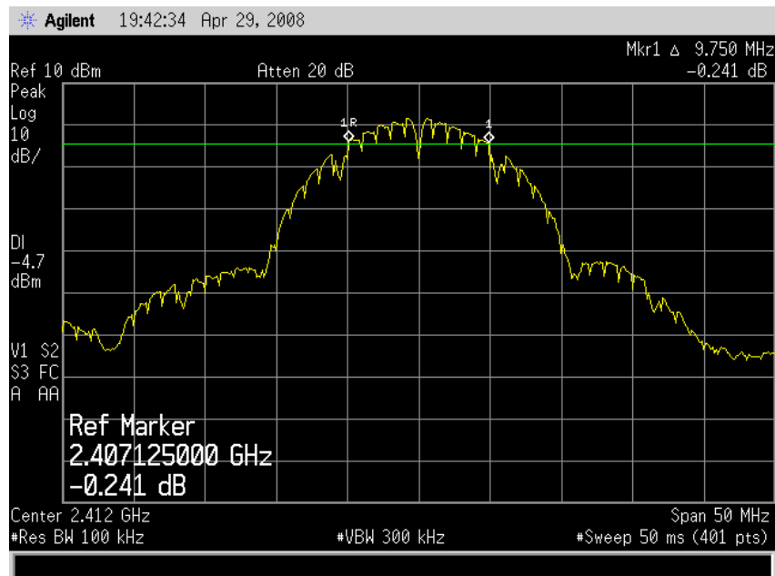
Plot 2 - Channel 1
