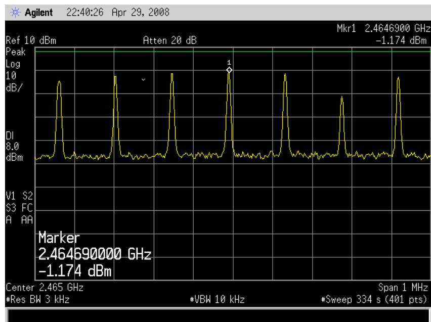
Plot 20 – Channel 2
