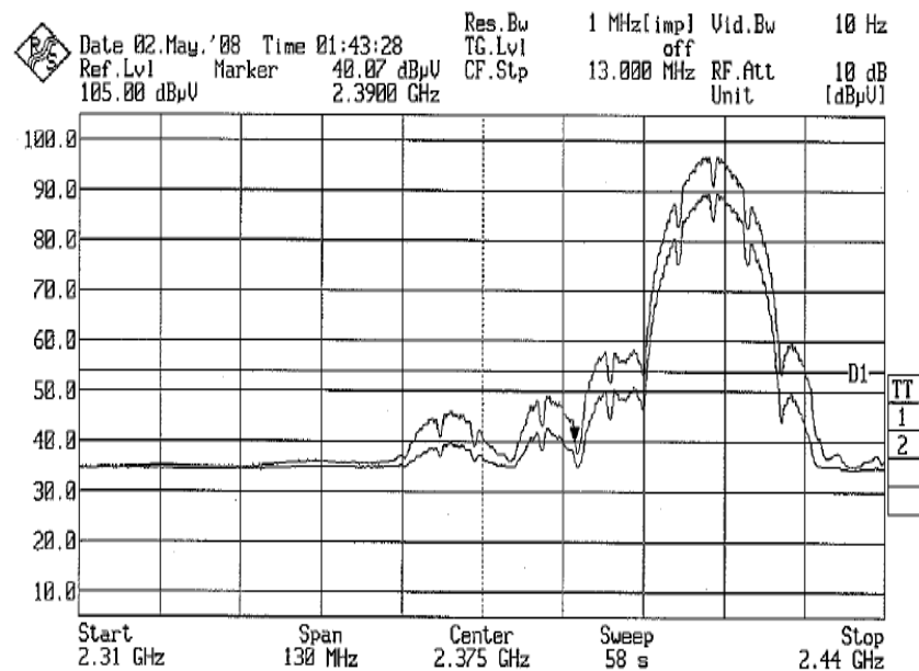
Plot 15 – Average Plot at Lower Band Edge at 2.4000GHz
