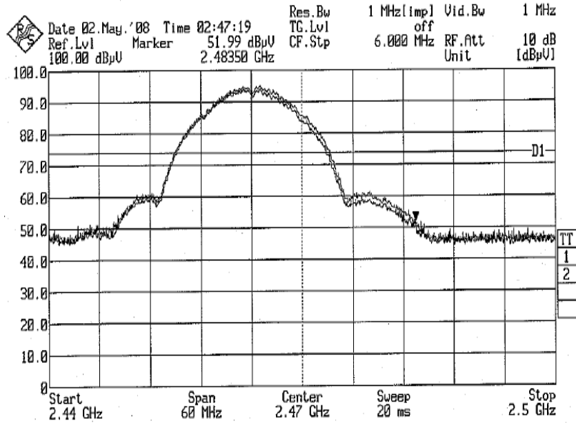
Plot 16 – Peak Plot at Upper Band Edge at 2.4835GHz
