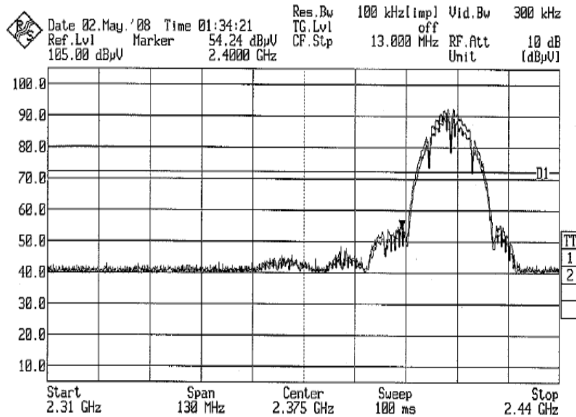
Plot 12 – Lower Band Edge at 2.4000GHz
