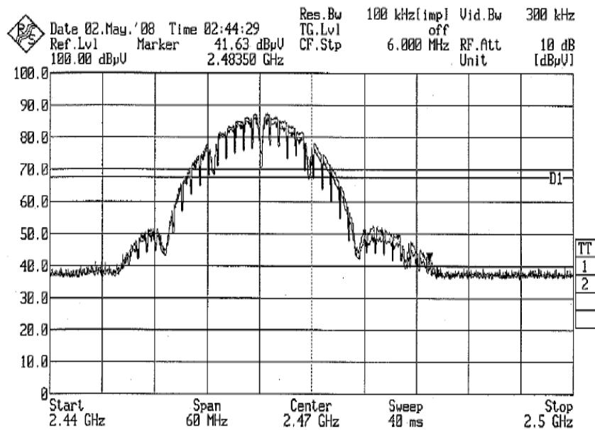
Plot 13 – Upper Band Edge at 2.4835GHz
