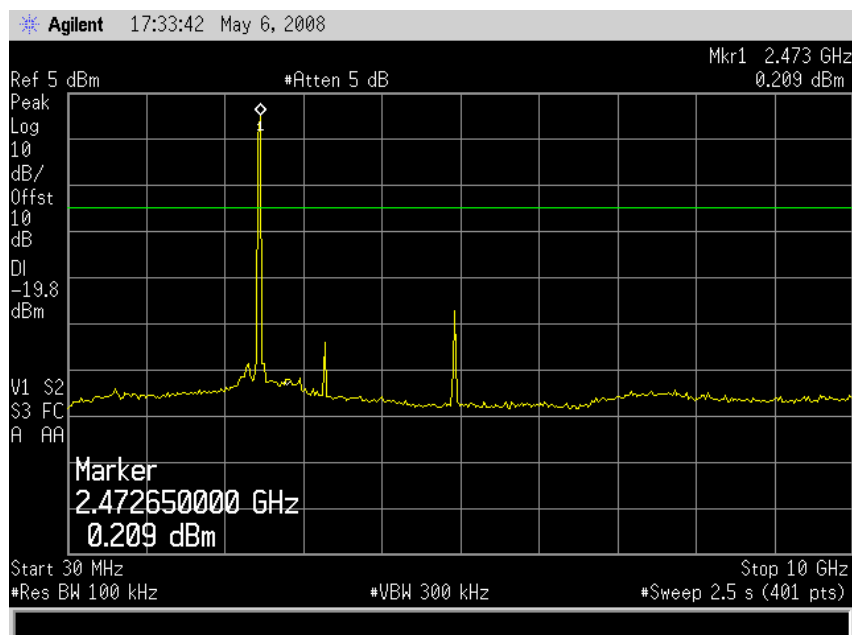
Plot 8 – Channel 2
