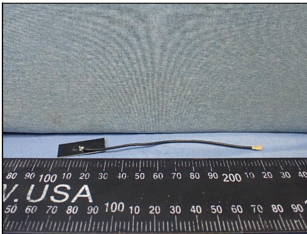
Antenna 2 (Brand: WHAYU / Model: 56-001-000044Z)
