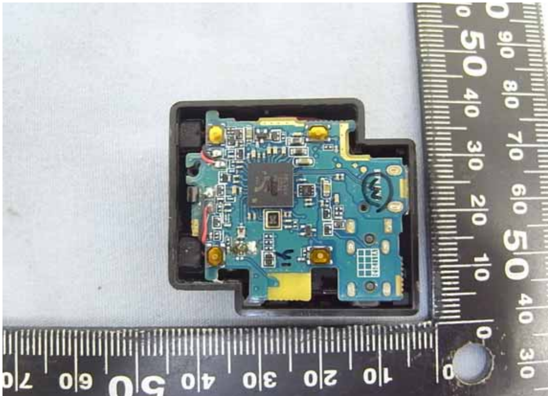
Figure 12 Internal View
