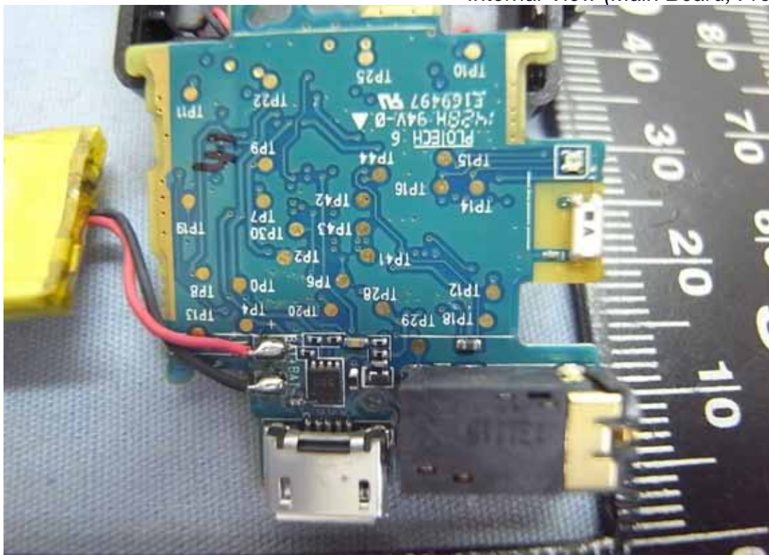
Figure 14 Internal View (Main Board, Front View)
