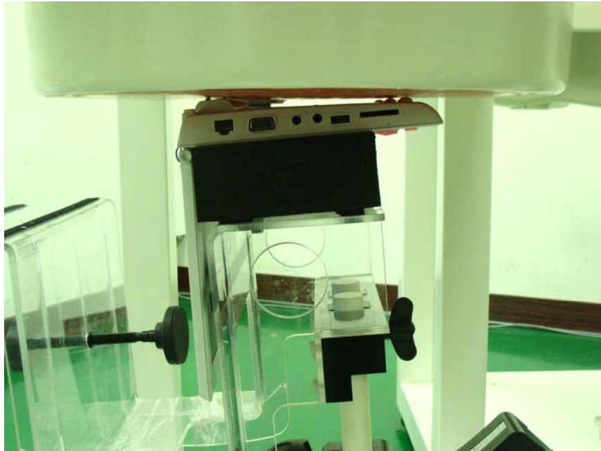
Bottom of the DUT with 0 cm Gap for Battery 1
