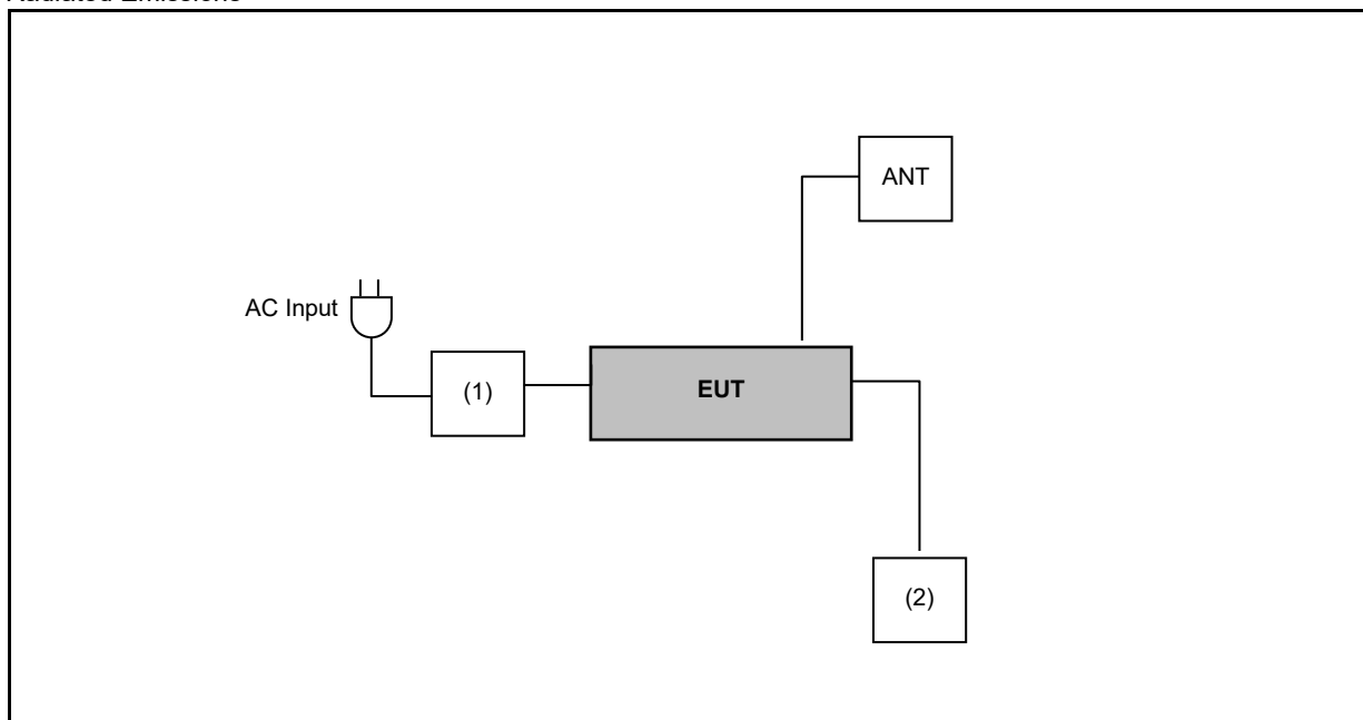
Radiated Emissions
