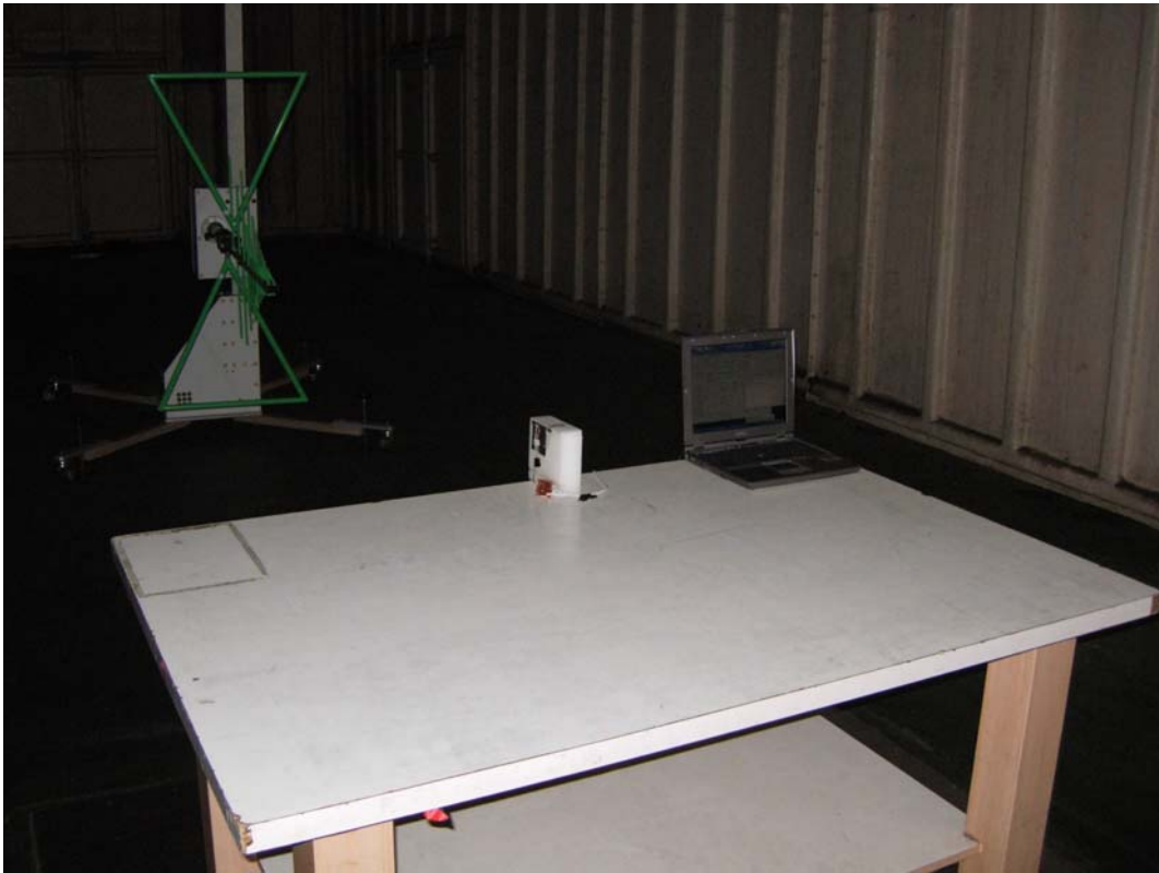
Back View of Radiated Test - Shielding C (Z-axis)
