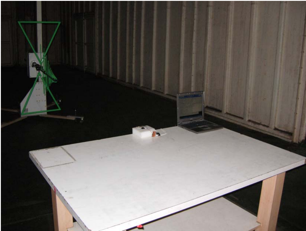
Back View of Radiated Test - Shielding B (X-axis)
