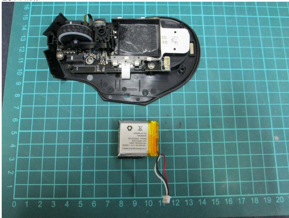
(10) EUT Photo (Li-ion Rechargeable Battery)
