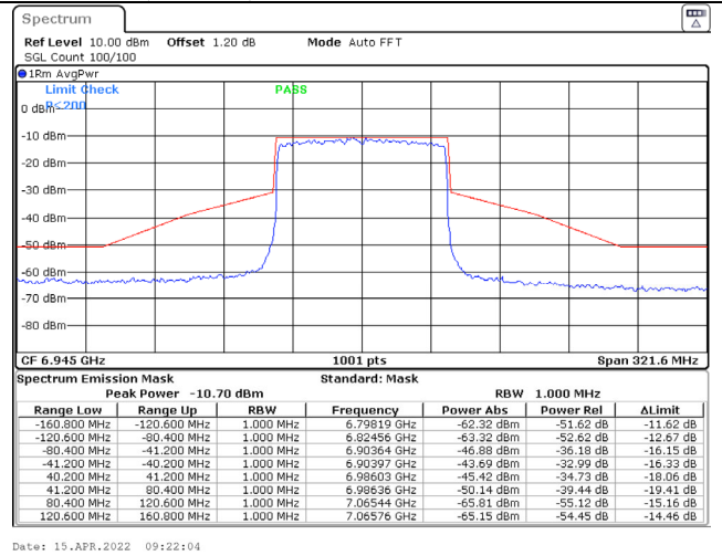
802.11ax (80MHz) / 6945MHz / Chain D / NSS-1
