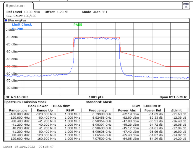
802.11ax (80MHz) / 6945MHz / Chain B / NSS-1
