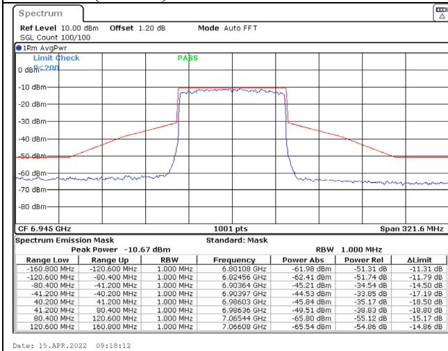
802.11ax (80MHz) / 6945MHz / Chain A / NSS-1
