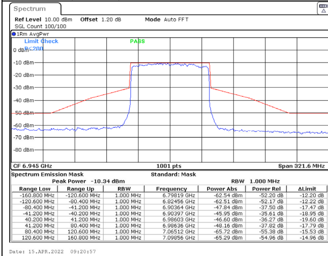
802.11ax (80MHz) / 6945MHz / Chain C / NSS-1
