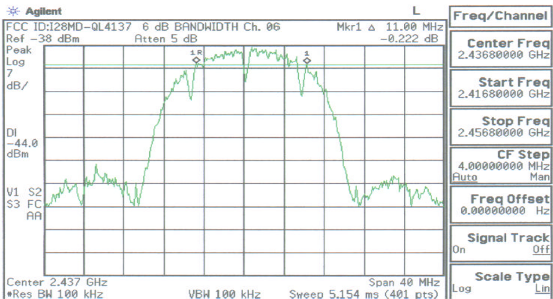
Plot A-2. 6dB Bandwidth Plot – Ch.6
