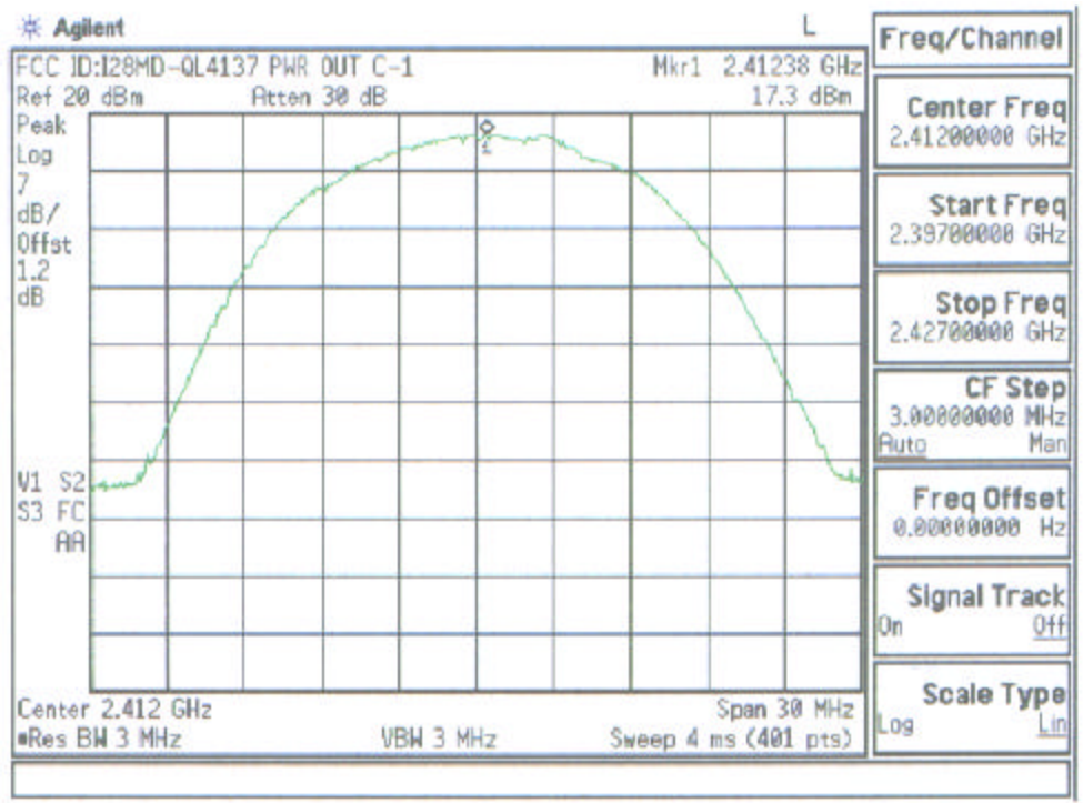
Plot A-4. Max. Peak Output Power Plot – Ch.1
