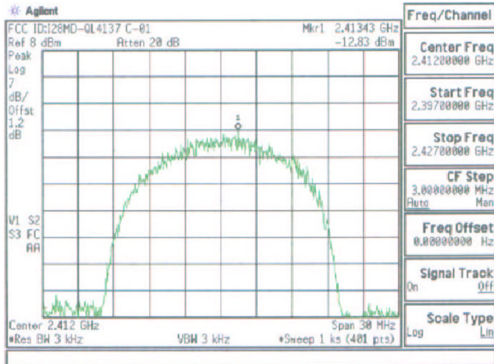
Plot A-7. Max. Power Density Plot – Ch.1
