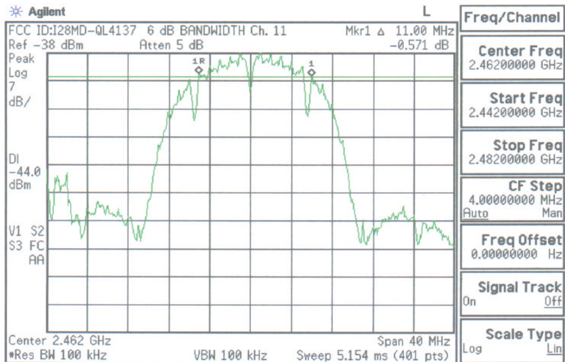
Plot A-3. 6dB Bandwidth Plot – Ch.11
