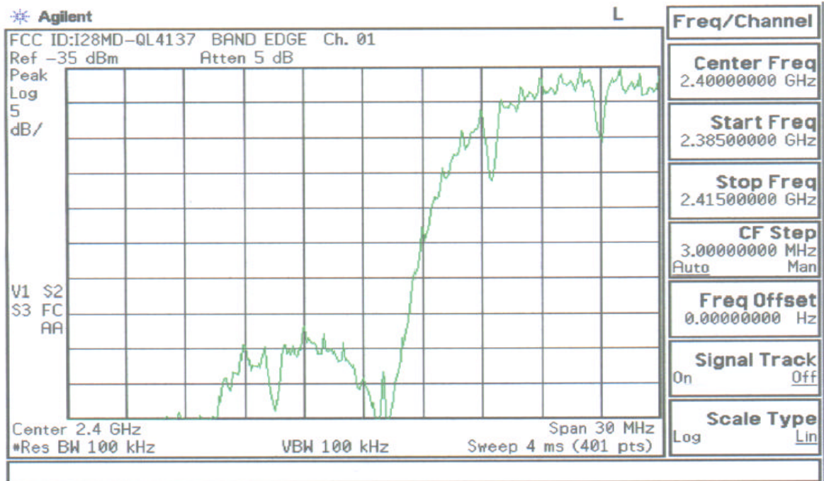
Plot A-10. BandEdge Plot – Ch.1
