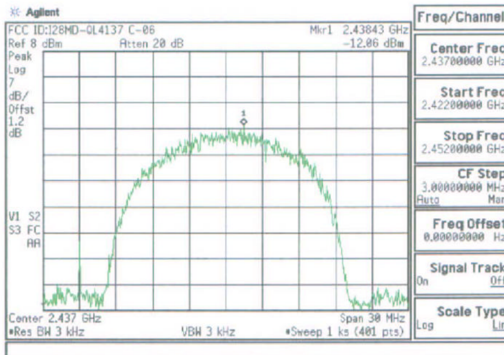
Plot A-8. Max. Power Density Plot – Ch.6
