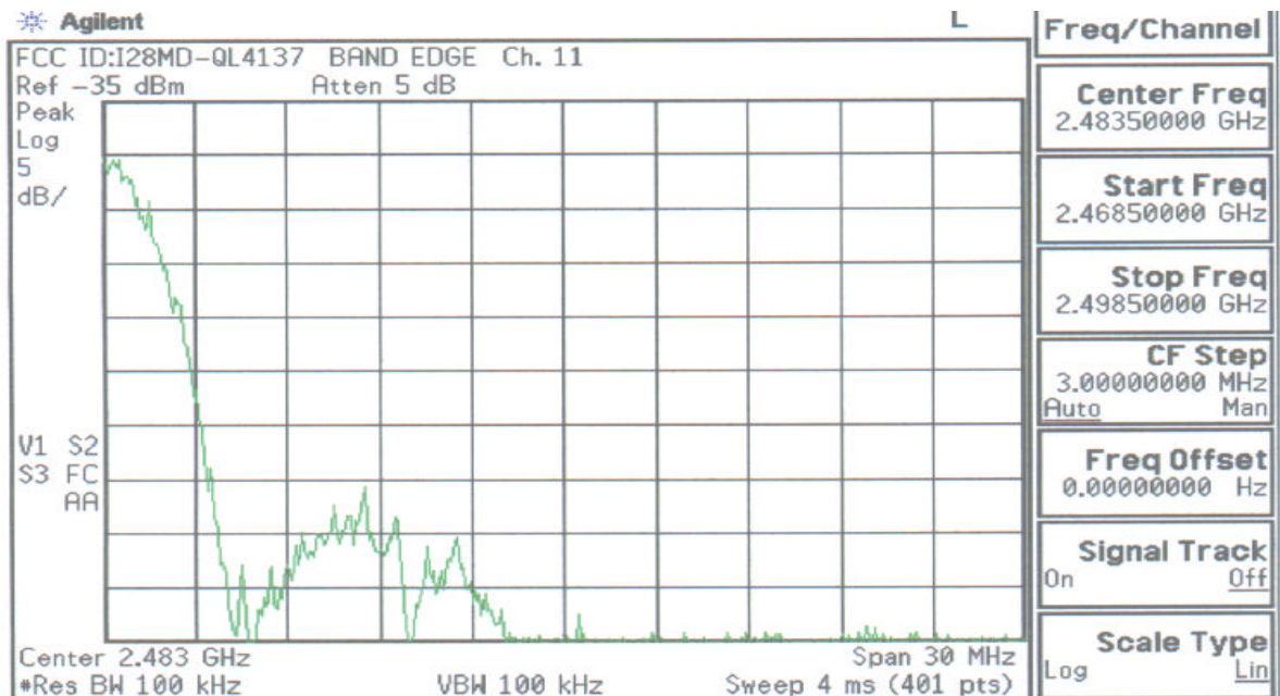
Plot A-12. BandEdge Plot – Ch.11
