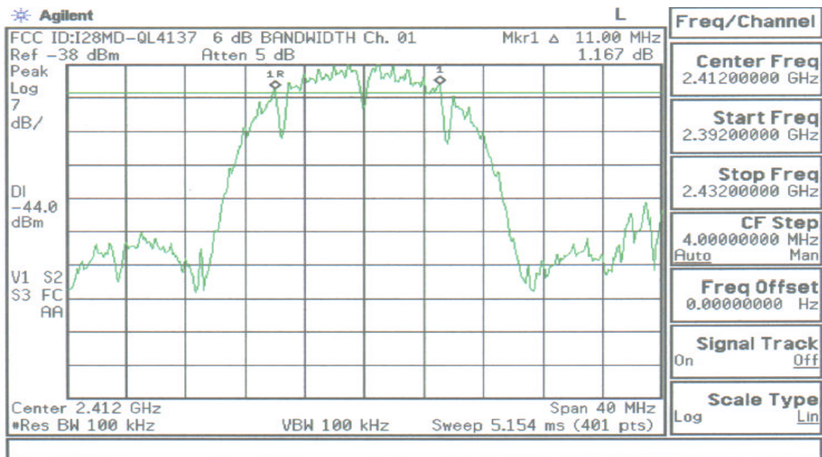
Plot A-1. 6dB Bandwidth Plot – Ch.1
