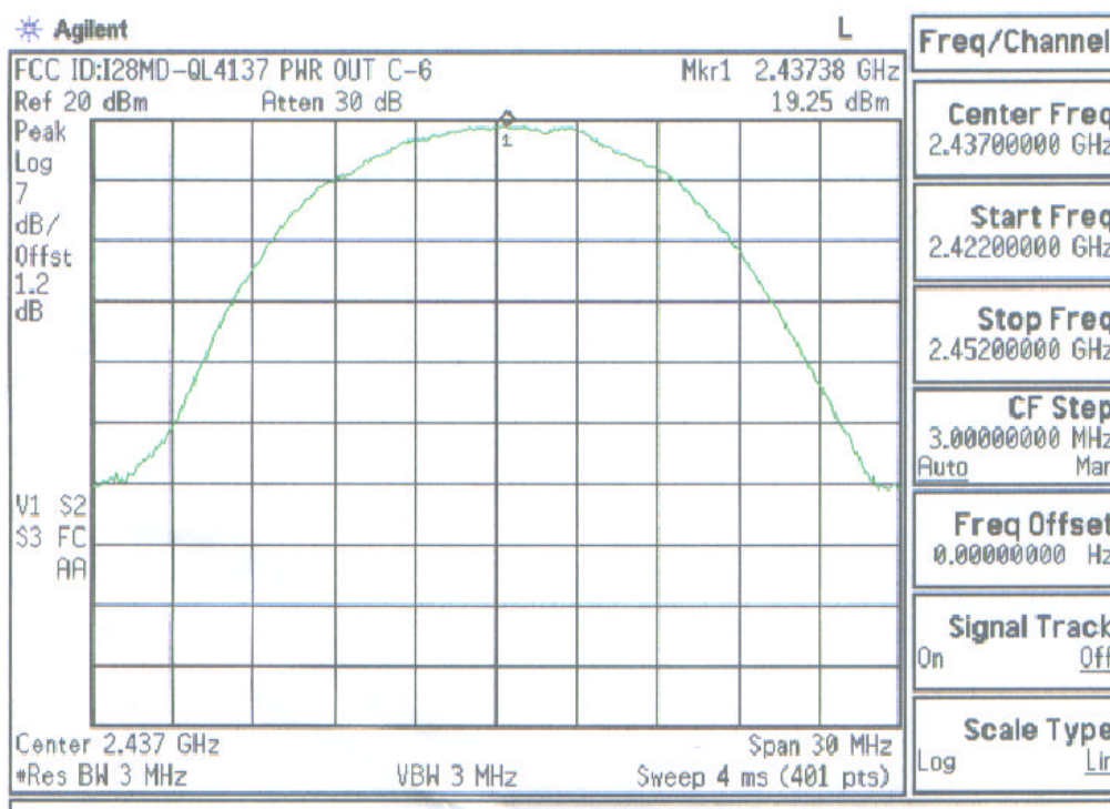
Plot A-5. Max. Peak Output Power Plot – Ch.6
