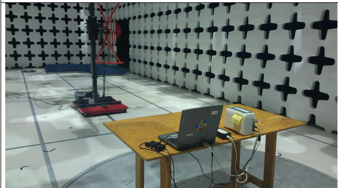
Radiated Emission Test Setup (below 1GHz) – Rear View
