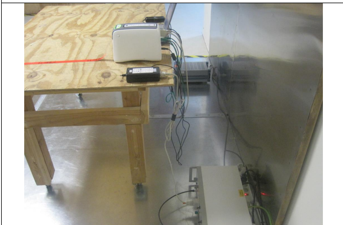
Conducted Emission Test Setup – Rear View
