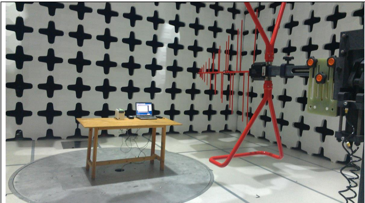
Radiated Emission Test Setup (below 1GHz) - Front View
