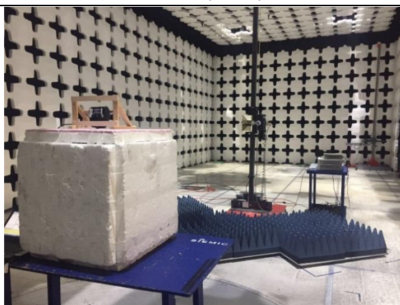
Radiated Emissions (>1GHz) – Rear View (EUT vertical)
