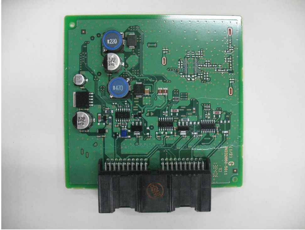
Component Side
