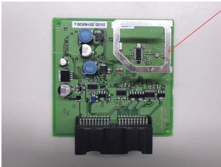
Component side
